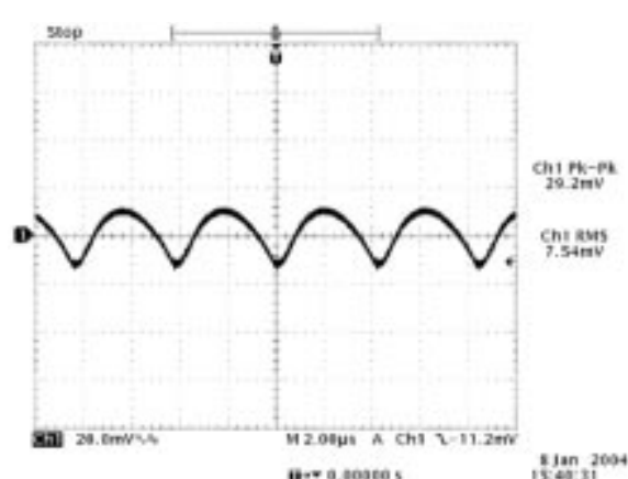
Ripple and noise at full load and 12Vdc input, 1.2Vdc output and Ta=25° C
