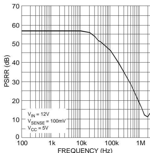
Fig. 19 Supply Rejection
