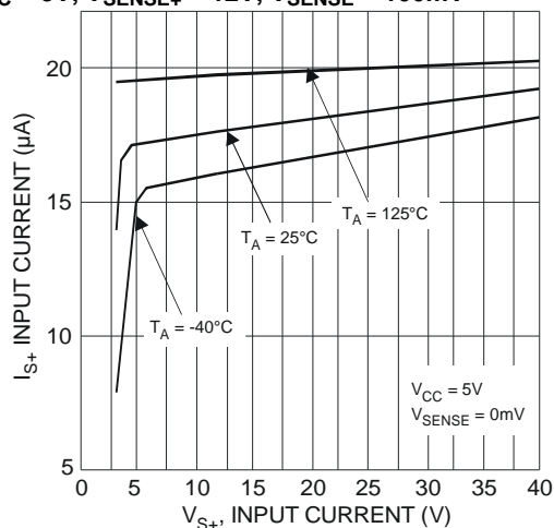
Fig. 2 Input Current
