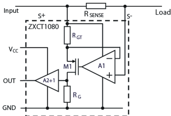
Fig. 20 Typical Configuration of ZXCT1080
