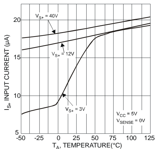
Fig. 3 Input Current
