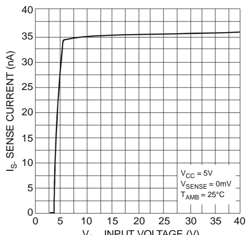
Fig. 4 Sense Current
