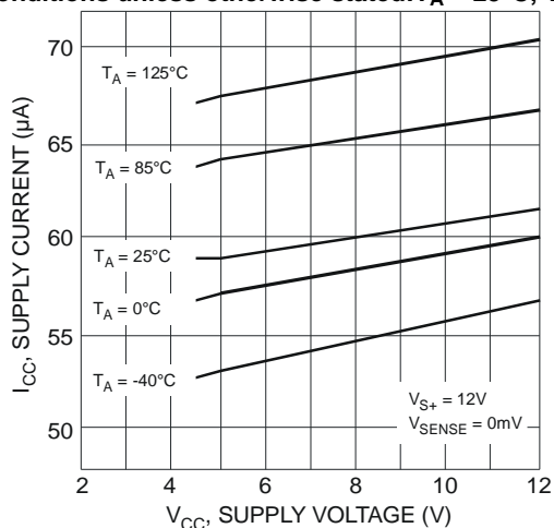
Fig. 1 Supply Current
