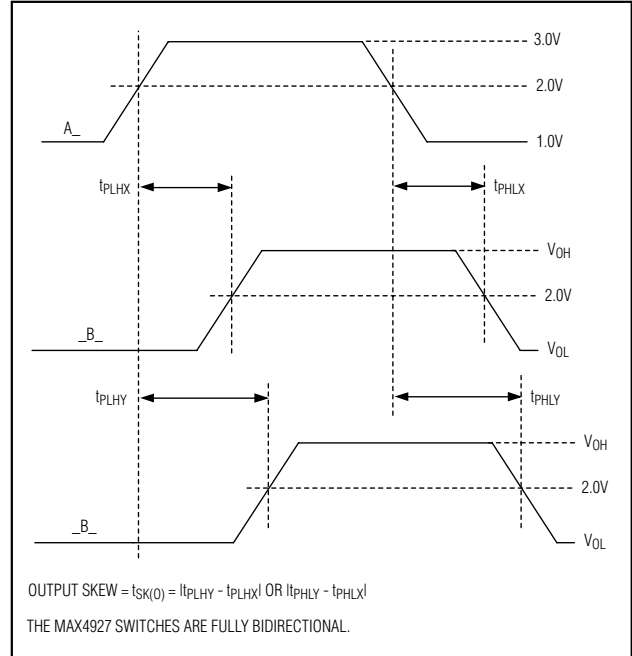
Figure 4. Output Skew
