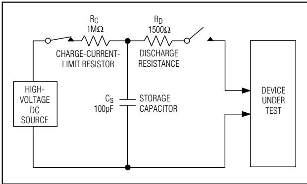
Figure 5a. Human Body ESD Test Model
