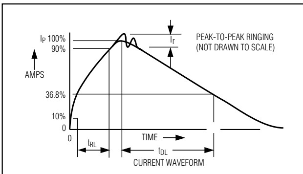
Figure 5b. Human Body Current Waveform
