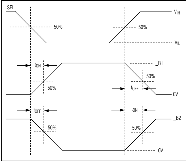
Figure 2. Turn-On and Turn-Off Times
