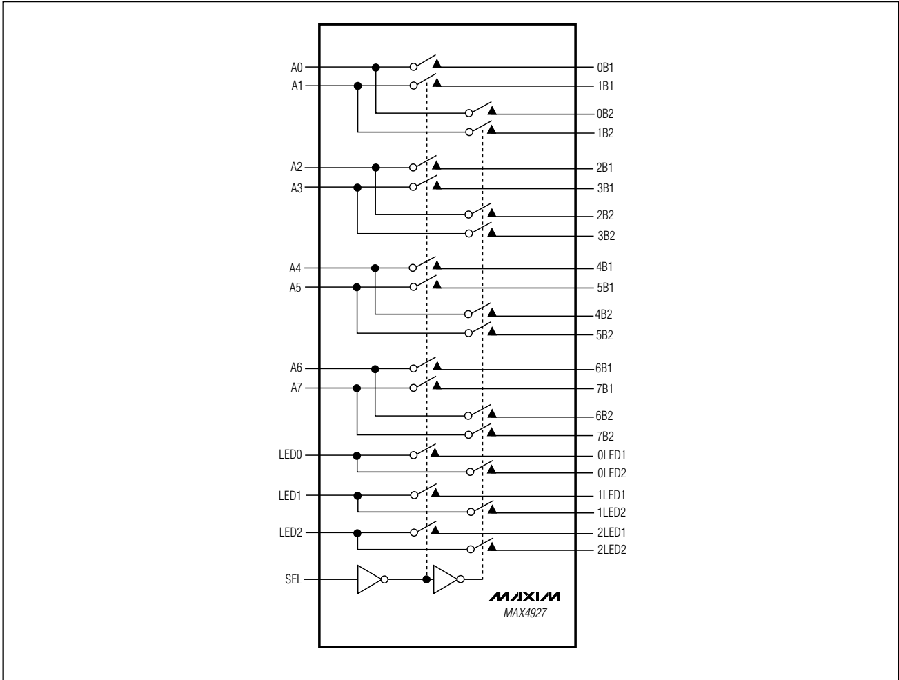
Functional Diagram
