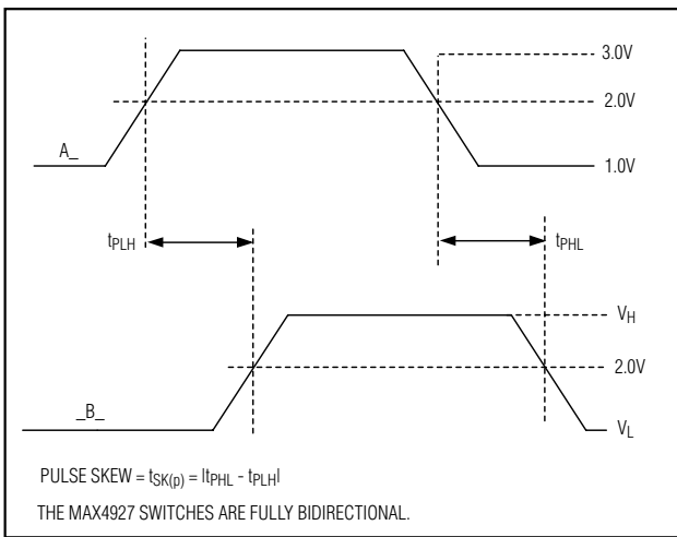
Figure 3. Propagation Delay Times
