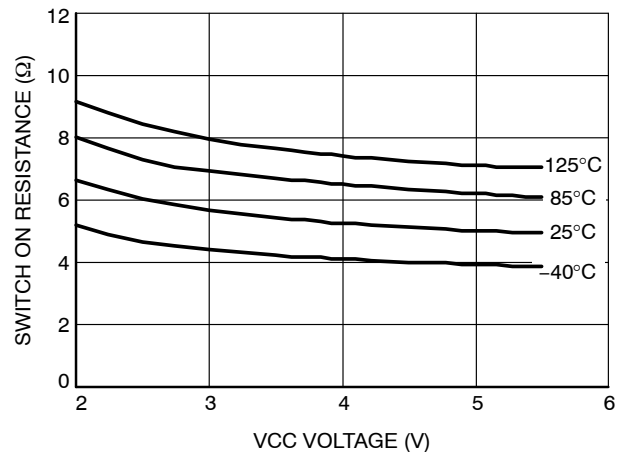
Figure 8. Switch On-resistance vs. VCC
