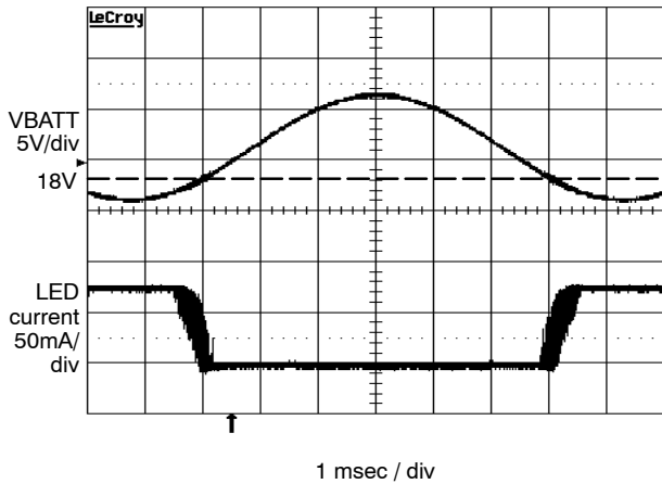
Figure 3. VBATT Overtolerance Detection Amplitude between 16 V and 26 V
