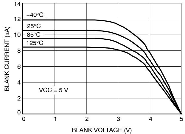
Figure 6. BLANK Pull-up Current vs. Input Voltage
