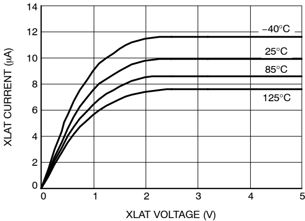
Figure 5. XLAT Pull-down Current vs. Input Voltage
