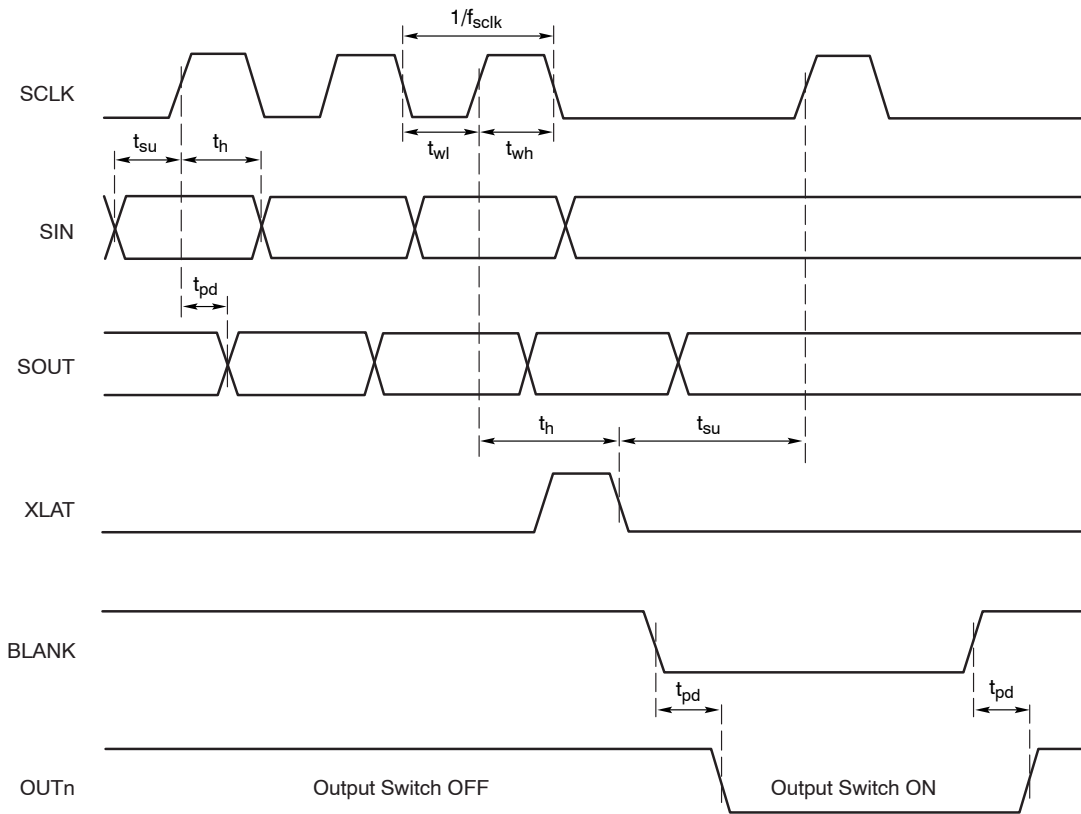
Figure 13. Timing Diagram
