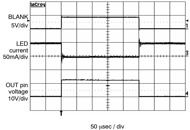
Figure 4. BLANK and Output Waveform
