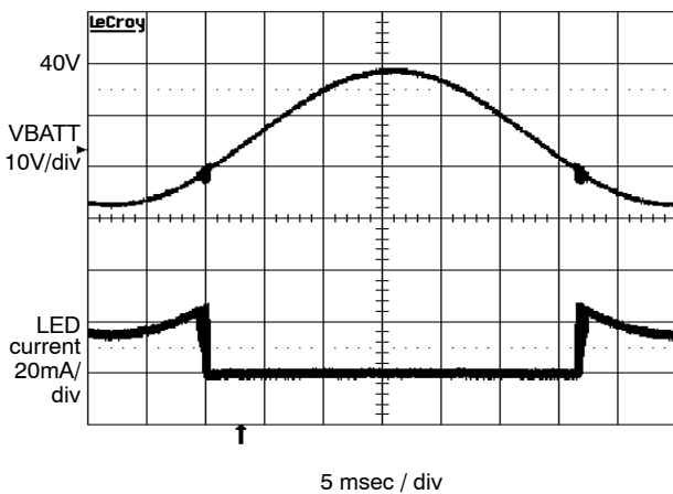
Figure 7. VBATT Load Dump
