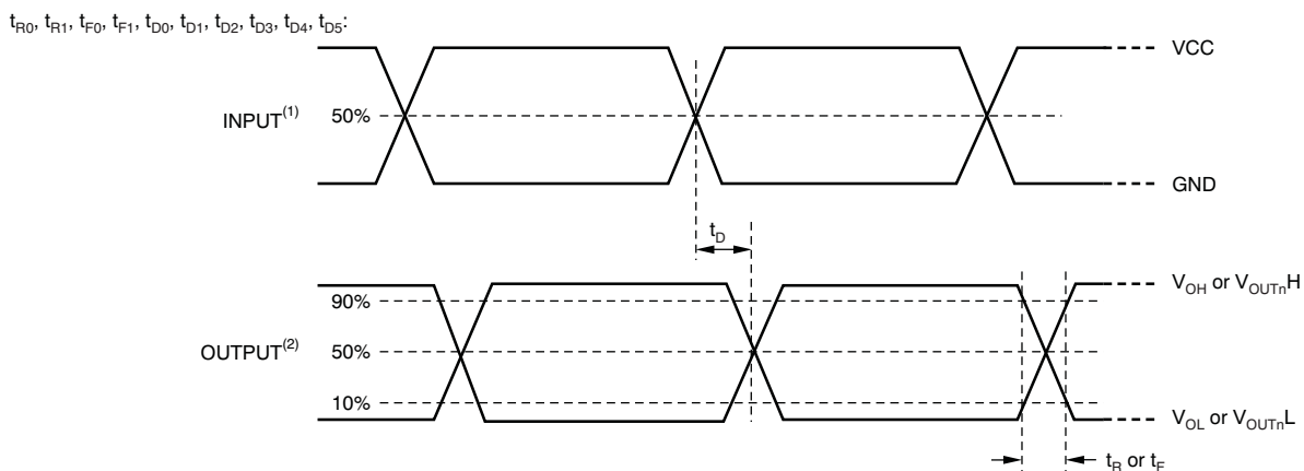
Figure 9. Input Timing
