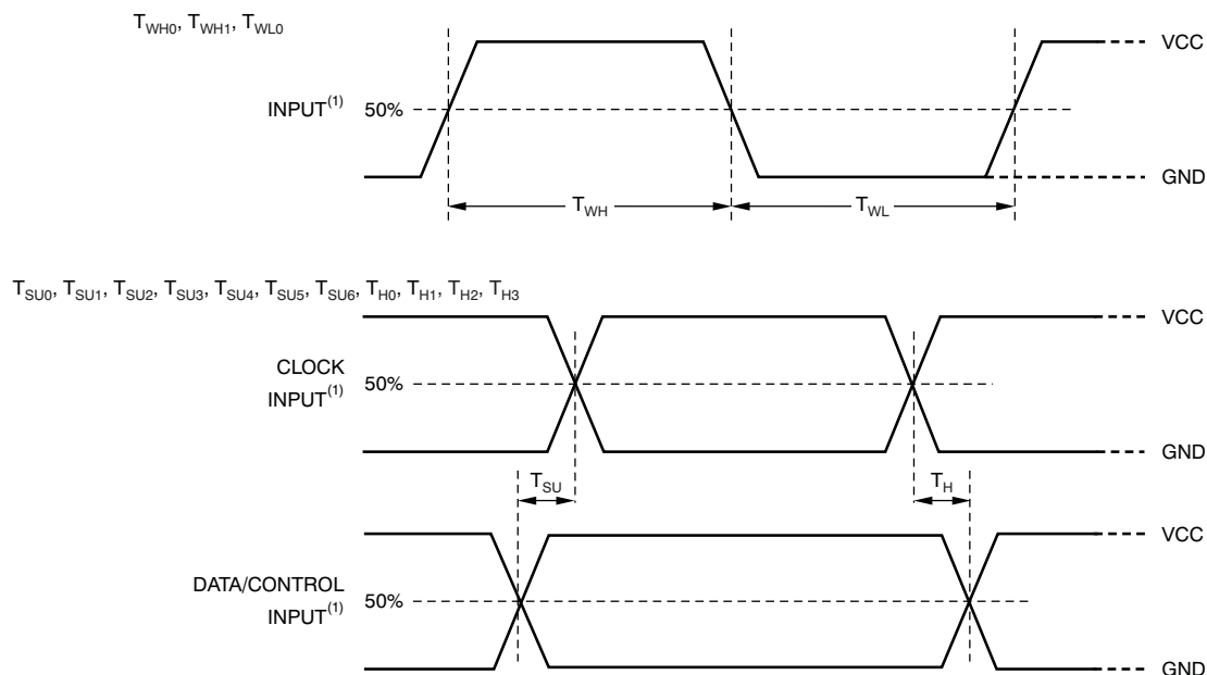
Figure 9. Input Timing
