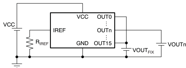
Figure 8. Constant Current Test Circuit for OUTn
