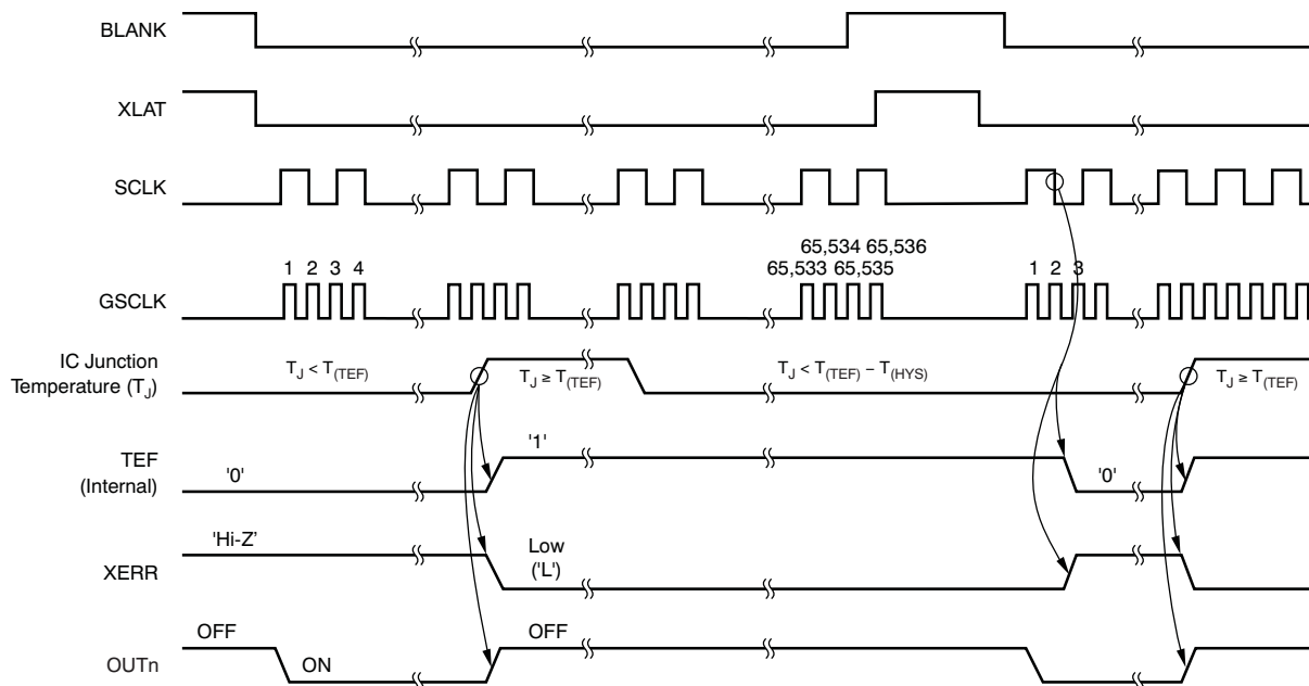
Figure 33. TEF/TSD/XERR timing
