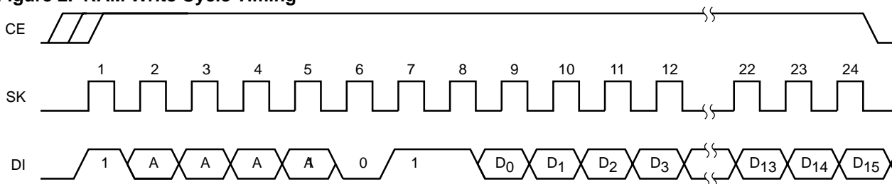
Figure 2. RAM Write Cycle Timing
