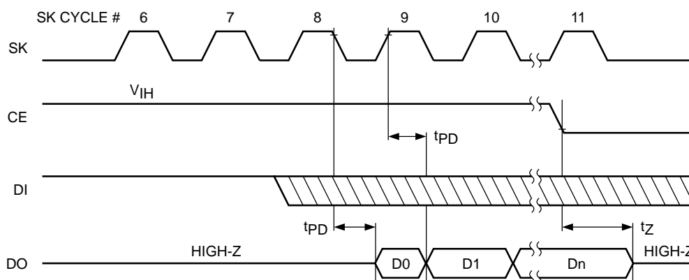
Figure 3. Read Cycle Timing
