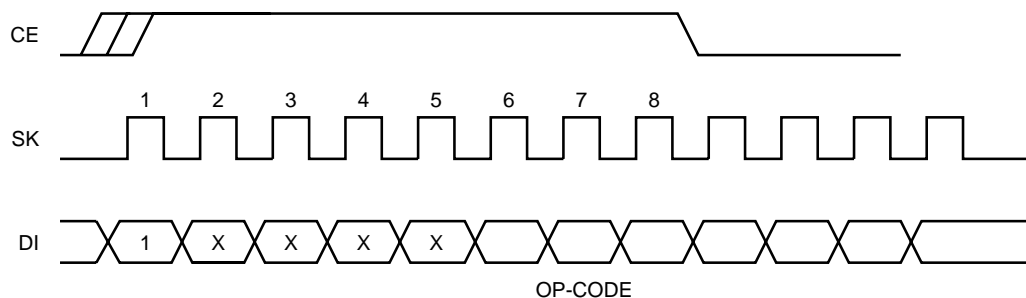
Figure 7. Non-Data Operations
