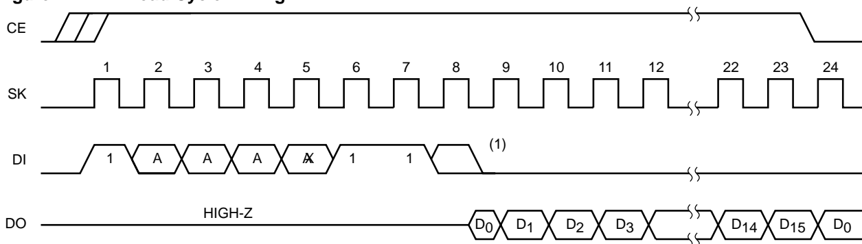
Figure 1. RAM Read Cycle Timing
