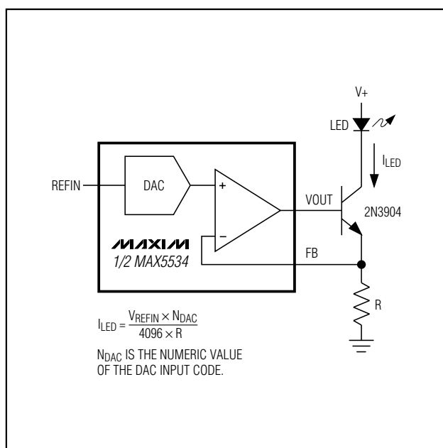
Figure 4. Programmable Current Source Driving an LED
