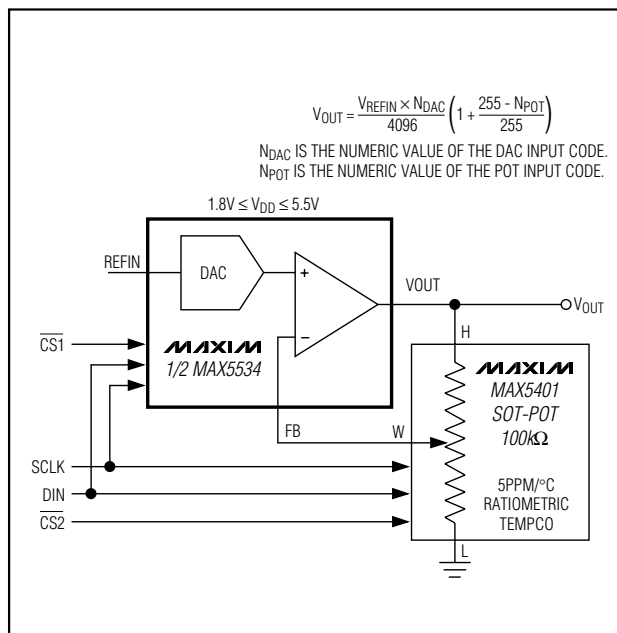
Figure 9. Software-Configurable Output Gain
