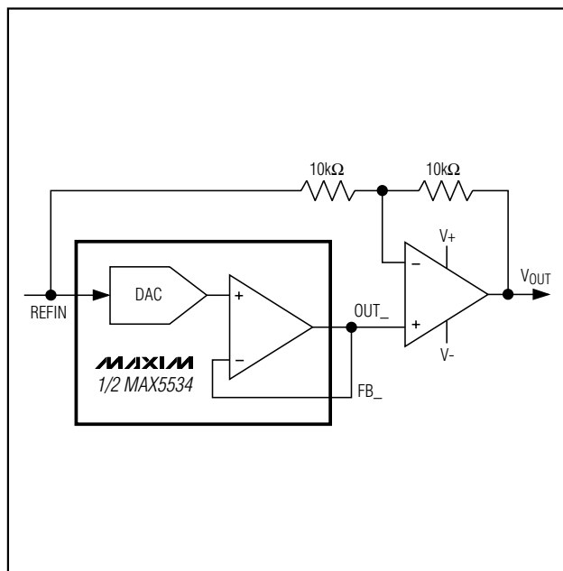
Figure 7. Bipolar Output Circuit
