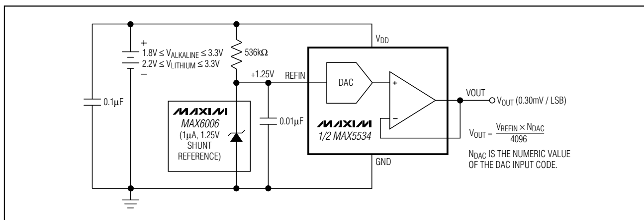
Figure 3. Portable Application Using Two Alkaline Cells or One Lithium Coin Cell
