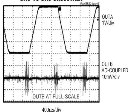
DAC-TO-DAC CROSSTALK
