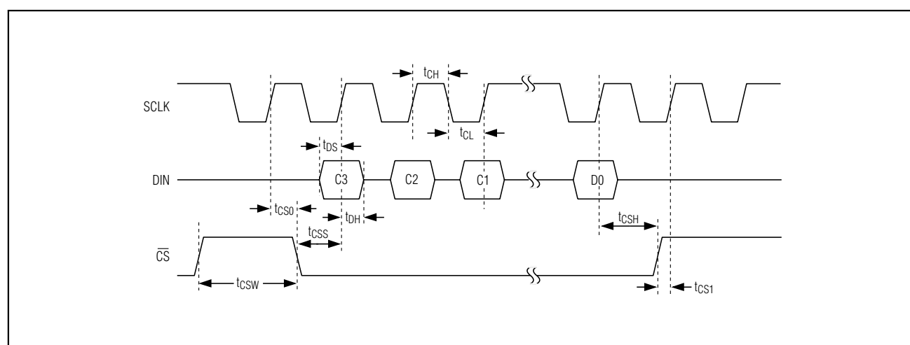
Figure 1. Timing Diagram
