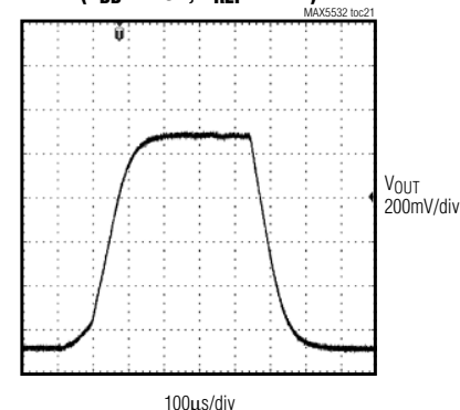
OUTPUT LARGE-SIGNAL STEP RESPONSE ( V_{DD} = 1.8V , V_{REF} = 1.2V )
