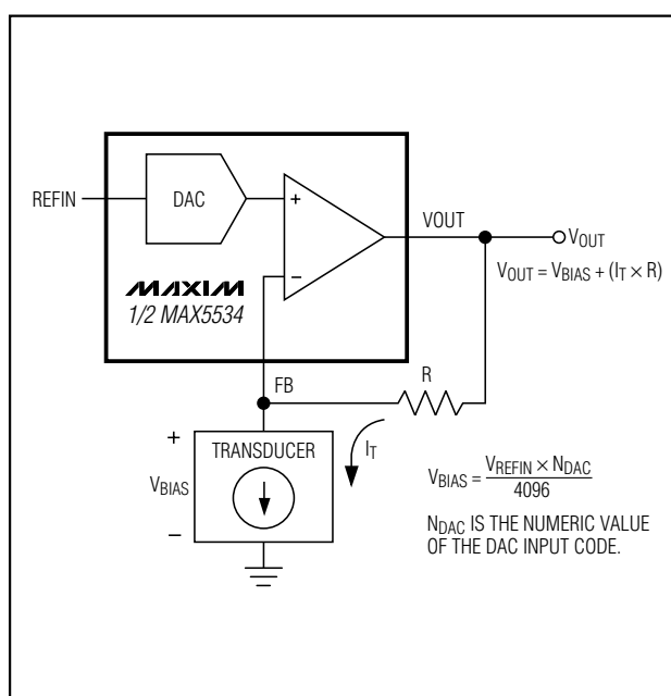
Figure 5. Transimpedance Configuration for a Voltage-Biased Current-Output Transducer
