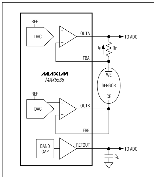
Figure 11. Driven Two-Electrode Potentiostat Application
