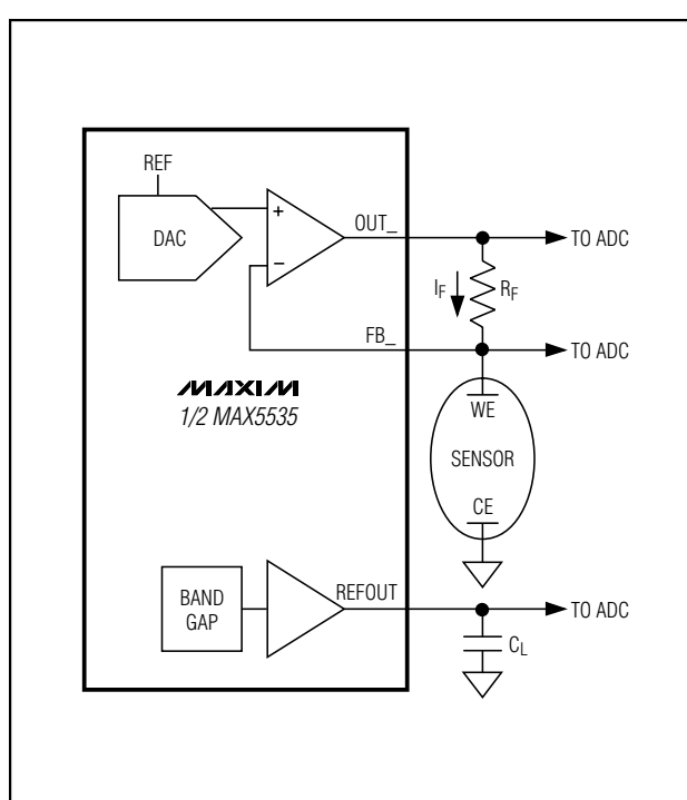
Figure 10. Self-Biased Two-Electrode Potentiostat Application
