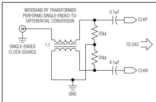
Figure 5. Differential Clock-Signal Generation
