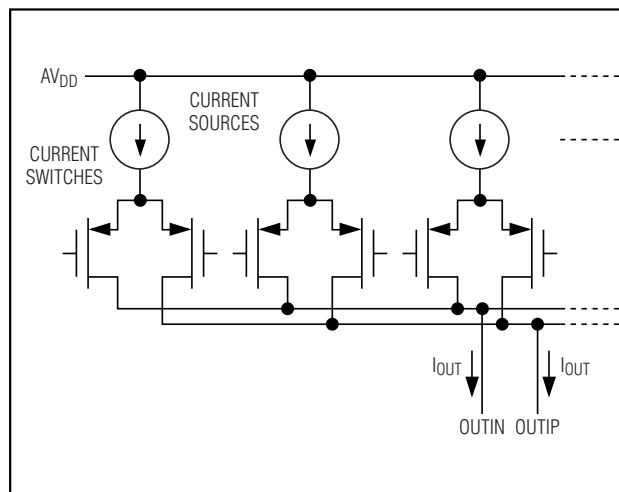
Figure 3. Simplified Analog Output Structure
