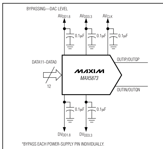
Figure 8. Recommended Power-Supply Decoupling and Bypassing Circuitry
