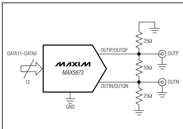
Figure 7. Differential Output Configuration
