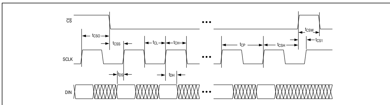
Figure 2. Timing Diagram
