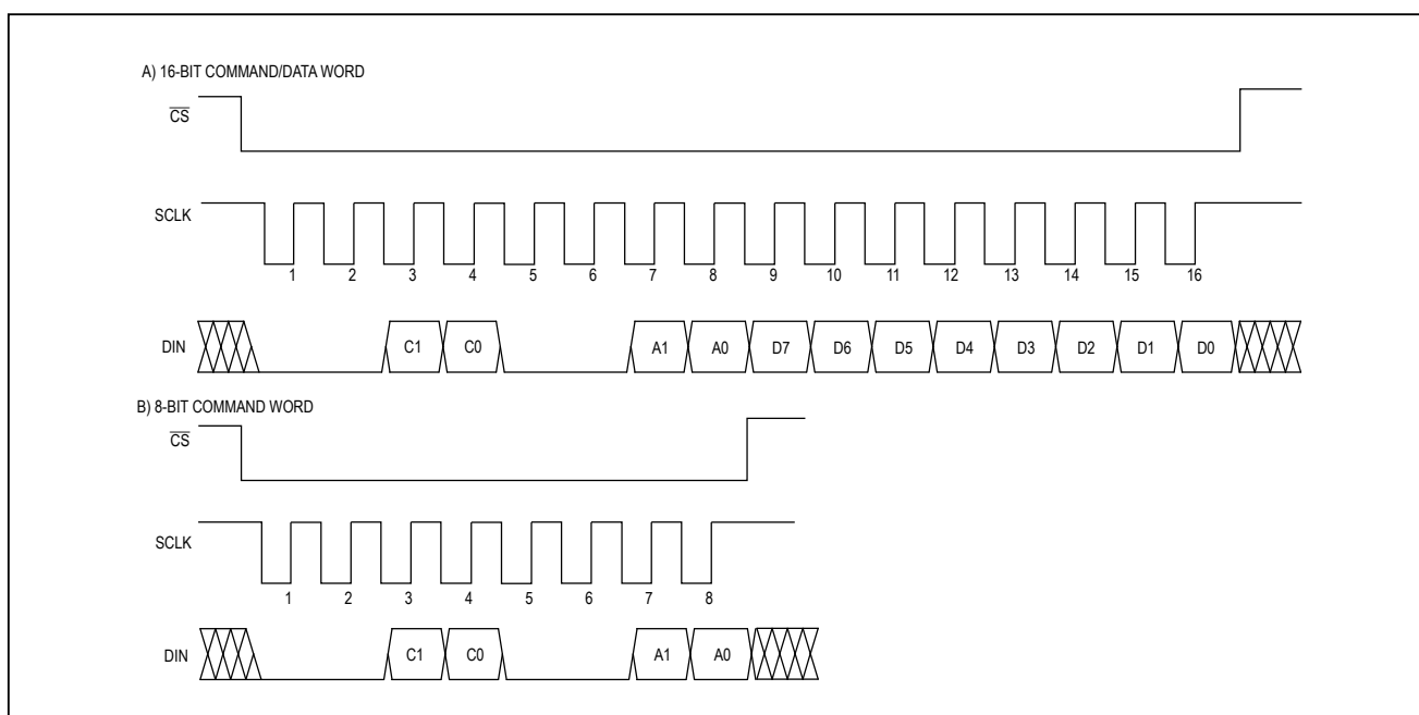
Figure 3. Digital-Interface Format
