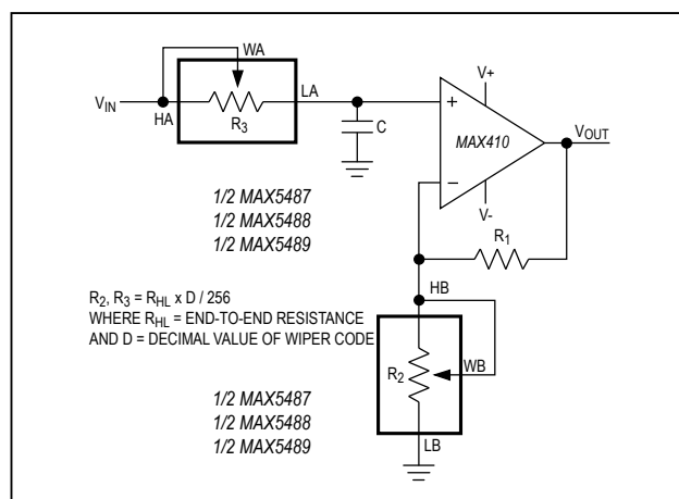
Figure 6. Programmable Filter
