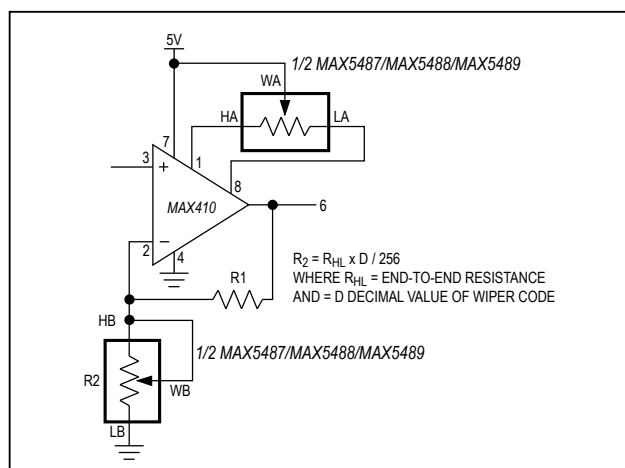
Figure 8. Offset Voltage and Gain Adjustment
