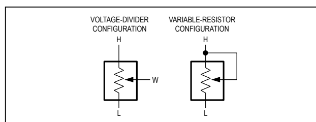
Figure 1. Voltage-Divider/Variable-Resistor Configurations
