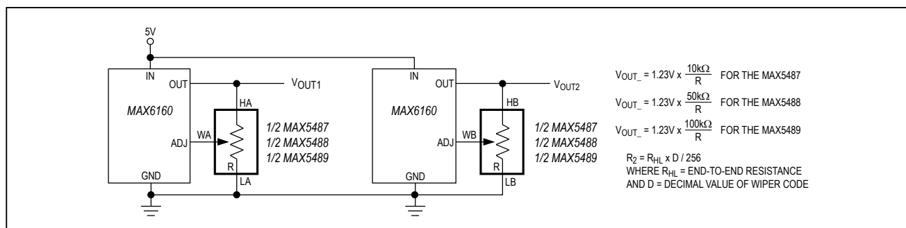
Figure 7. Adjustable Voltage Reference
