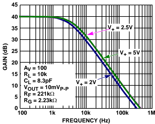
FIGURE 3. ISL28176 GAIN vs FREQUENCY vs SUPPLY VOLTAGE
