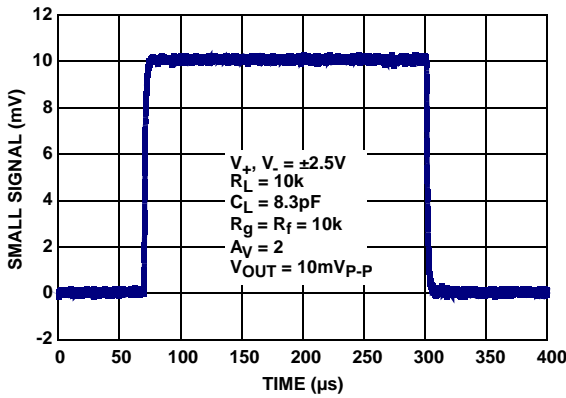
FIGURE 15. ISL28176 SMALL SIGNAL TRANSIENT RESPONSE
