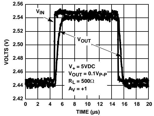
FIGURE 16. ISL28276, ISL28476 SMALL SIGNAL TRANSIENT RESPONSE
