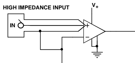
FIGURE 60. GUARD RING EXAMPLE FOR UNITY GAIN AMPLIFIER
