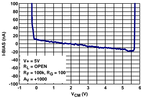
FIGURE 21. INPUT OFFSET CURRENT vs COMMON-MODE INPUT VOLTAGE
