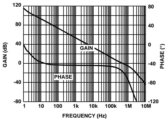
FIGURE 5. A_{VOL} vs FREQUENCY @ 100kΩ LOAD
