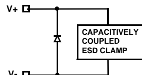
CIRCUIT 4
