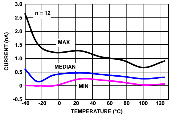
FIGURE 38. ISL28176 I_{BIAS}(-) vs TEMPERATURE V_S = \pm 1.2V
