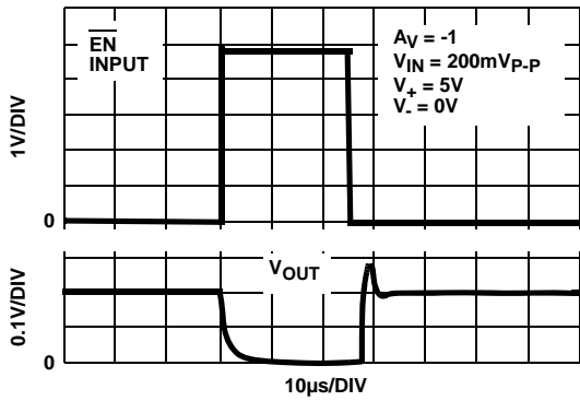
FIGURE 19. ISL28276 ENABLE TO OUTPUT DELAY TIME
