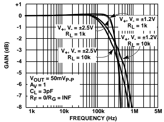
FIGURE 2. ISL28276, ISL28476 FREQUENCY RESPONSE vs SUPPLY VOLTAGE
