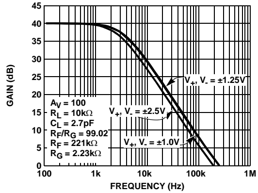
FIGURE 4. ISL28276, ISL28476 FREQUENCY RESPONSE vs SUPPLY VOLTAGE
