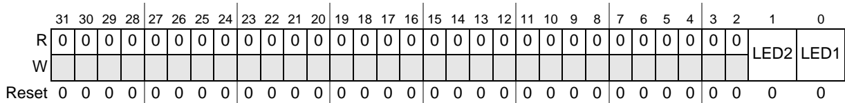
Figure 18. FPGA_LEDS Register
