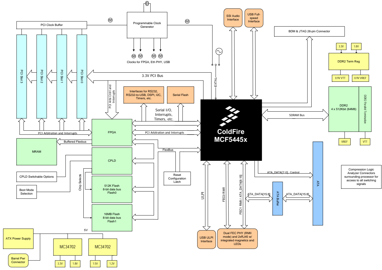
Figure 3. M54455EVB Block Diagram
