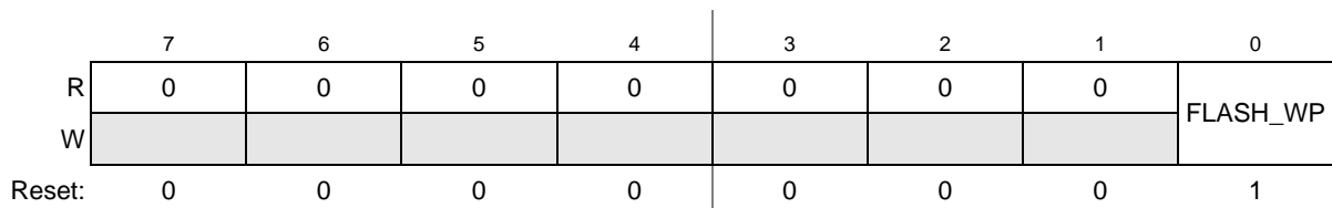
Figure 23. CPLD_FLASHCFG Register
