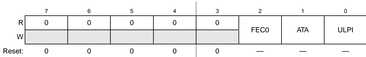
Figure 20. CPLD_CONTROL Register
