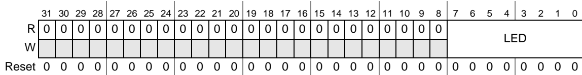
Figure 17. FPGA_7SEGMENT Register
