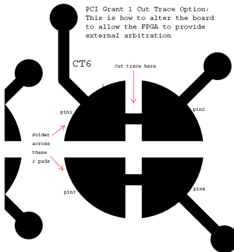
Figure 10. PCI Grant 1 Cut Trace Option—Use FPGA for Arbitration
