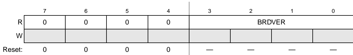
Figure 19. CPLD_VERSION Register
