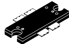
CASE 1484-04, STYLE 1 TO-272 WB-4 MRF5S4125NBR1
