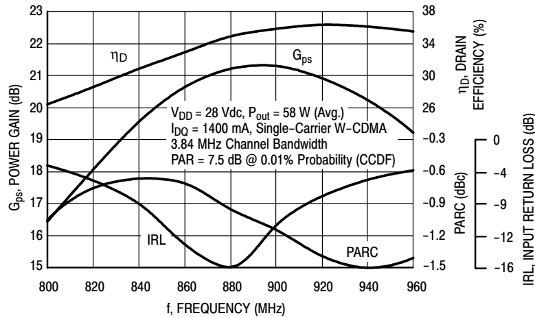
Figure 3. Single-Carrier W-CDMA Broadband Performance @ P_{out} = 58 Watts Avg.
