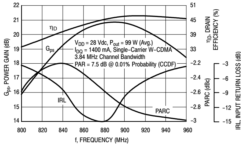
Figure 4. Single-Carrier W-CDMA Broadband Performance @ P_{out} = 99 Watts Avg.
