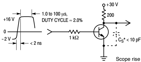
Figure 1. Turn-On Time
