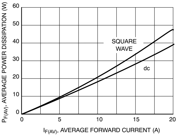
Figure 4. Power Dissipation
