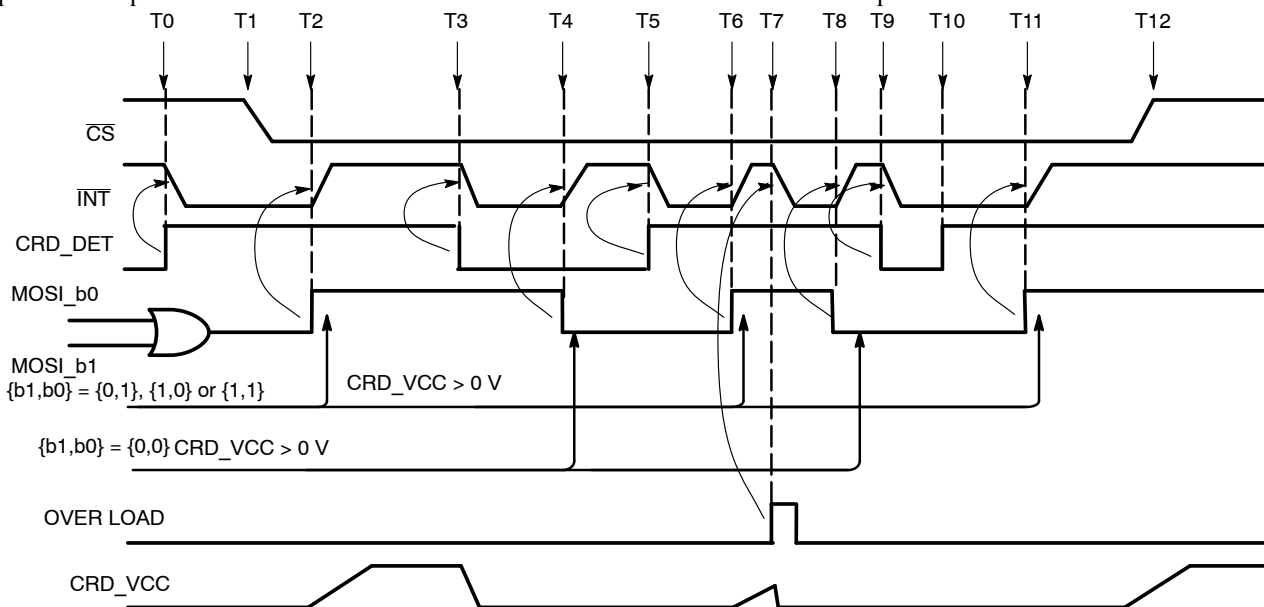
Figure 10. Basic Interrupt Function
