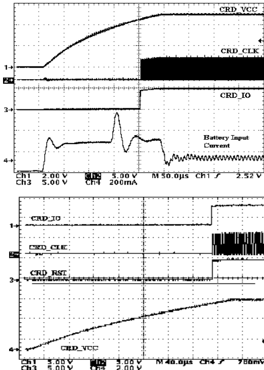
Figure 4. Measured Typical Startup CRD_VCC Sequence
