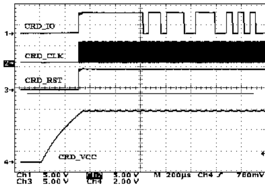
Figure 6. Figure 7: Start Up Sequence with ATR.
