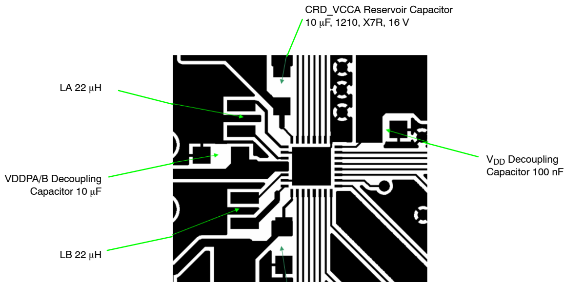
Figure 25. Example of PCB Device Implementation
