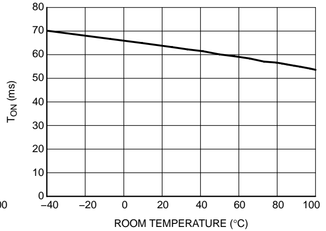
Figure 17. Turn On Time versus Room Temperature @ V BAT = 3.6 V, C BYP = 1 μF, C IN = 100 nF, R IN = 22 k, R F = 110 k
