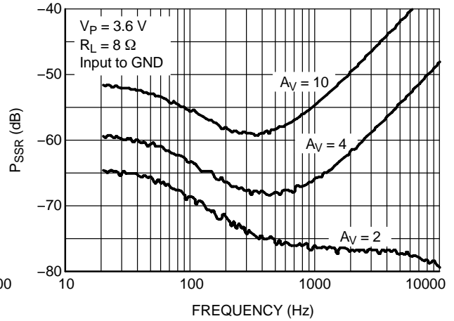
Figure 15. P SRR versus Frequency and Gain @ V P = 3.6 V
