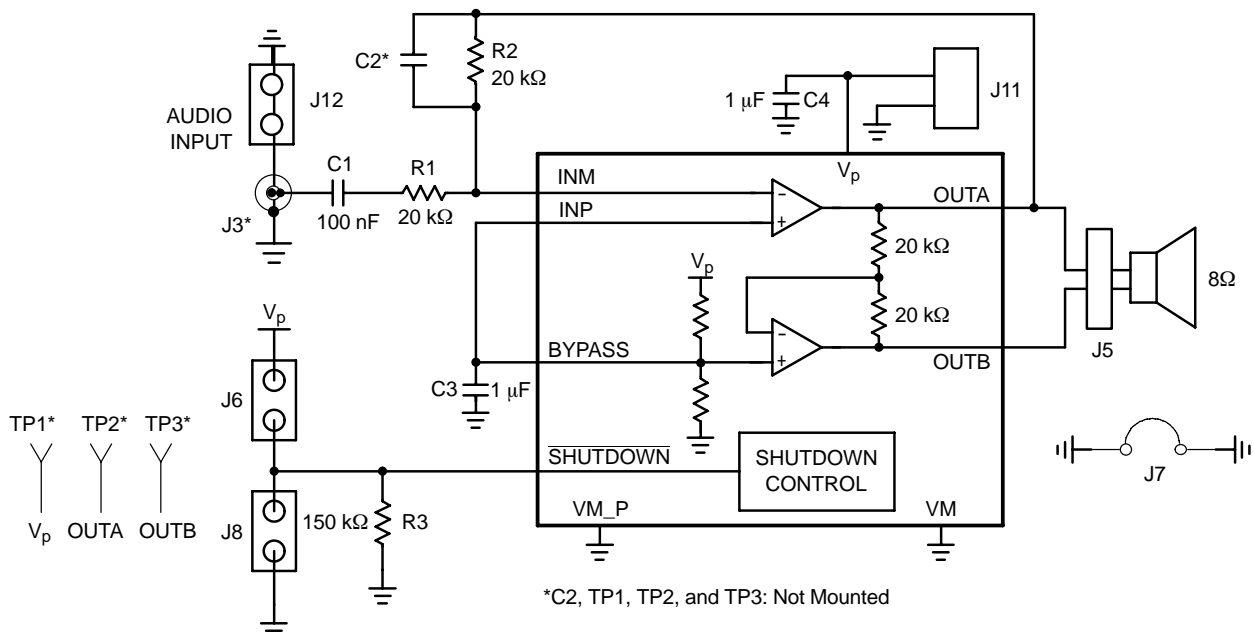
Figure 25. Schematic of the NCP2990 Demonstration Board
