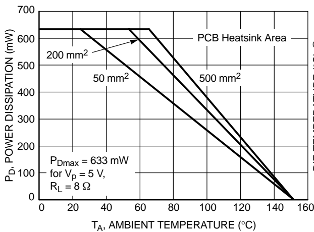
Figure 23. Power Derating - 9-Pin Flip-Chip CSP
