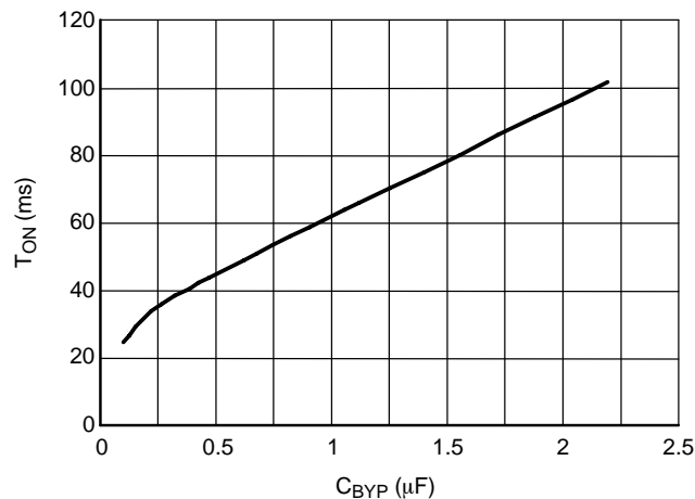
Figure 18. Turn On Time versus C BYP @ V BAT = 3.6 V, T A = +25°C, C IN = 100 nF, R IN = 22 k, R F = 110 k
