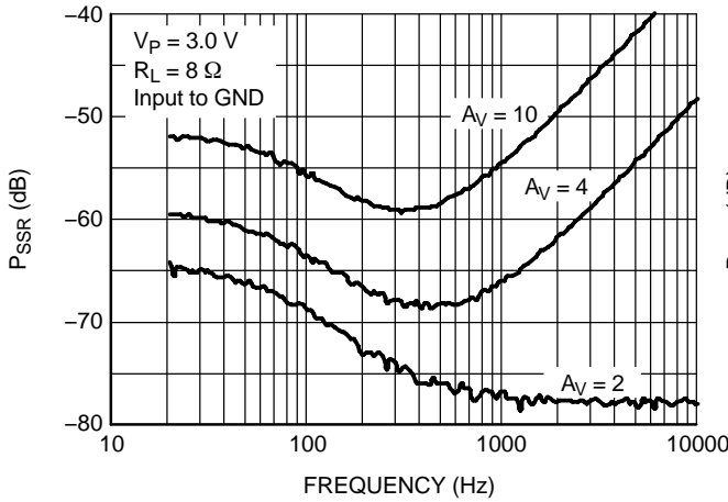
Figure 14. P SRR versus Frequency and Gain @ V P = 3.0 V
