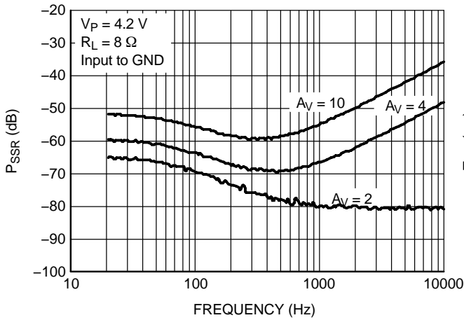
Figure 16. P SRR versus Frequency and Gain @ V P = 4.2 V
