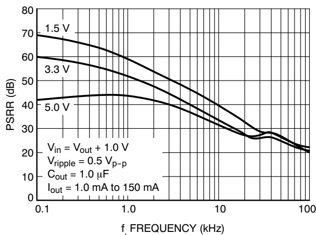
Figure 22. Power Supply Ripple Rejection vs. Frequency
