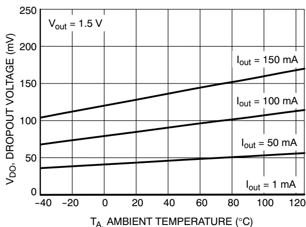
Figure 9. Dropout Voltage vs. Temperature (Over Current Range)
