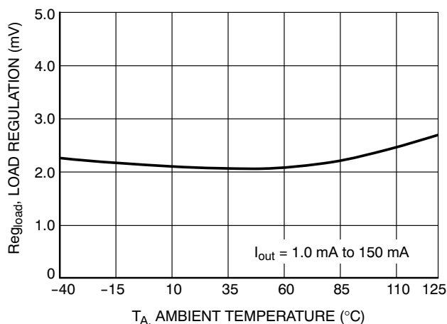
Figure 20. Load Regulation vs. Temperature
