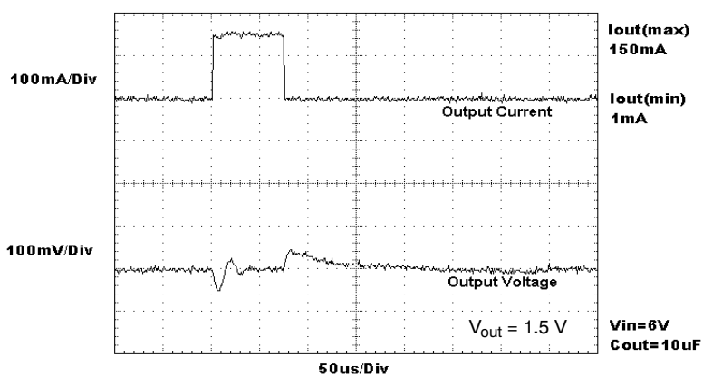
Figure 25. Load Transient Response (10 \mu\text{F} )
