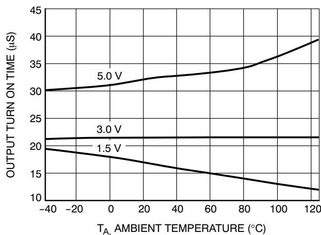
Figure 21. Output Turn On Time vs. Temperature
