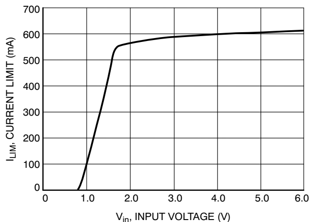
Figure 18. Current Limit vs. Input Voltage
