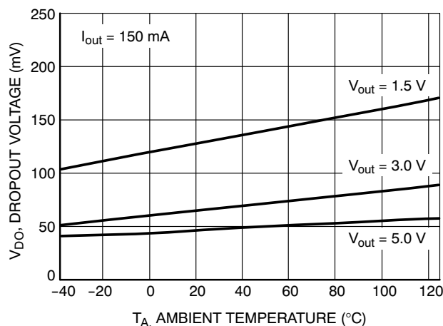
Figure 10. Dropout Voltage vs. Temperature (Over Output Voltage)
