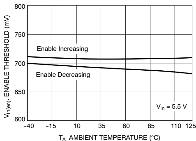
Figure 12. Enable Threshold vs. Temperature
