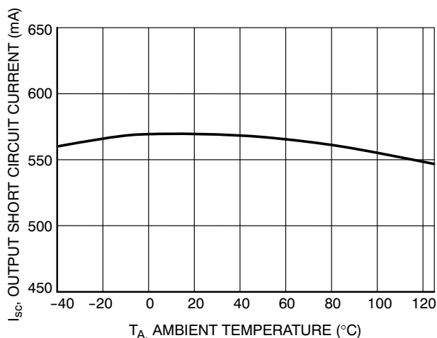
Figure 17. Output Short Circuit Current vs. Temperature
