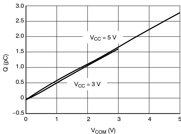
Figure 15. Charge Injection vs. COM Voltage
