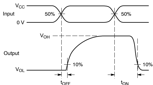
Figure 6. t_{ON}/t_{OFF}
