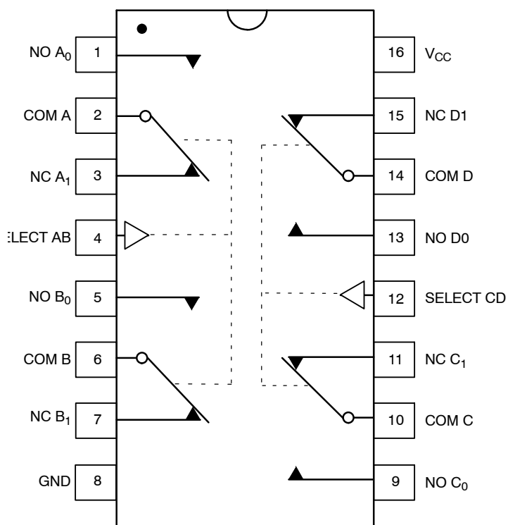
Figure 1. Logic Diagram
