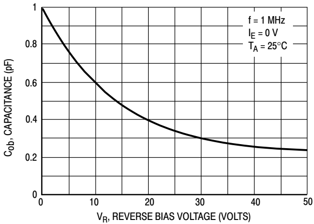
Figure 4. Output Capacitance
