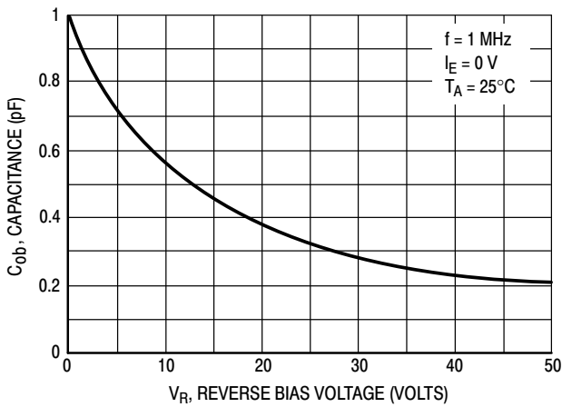
Figure 9. Output Capacitance
