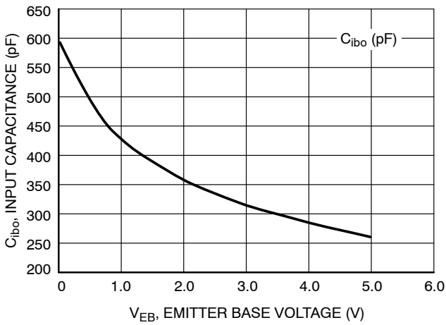
Figure 7. Input Capacitance
