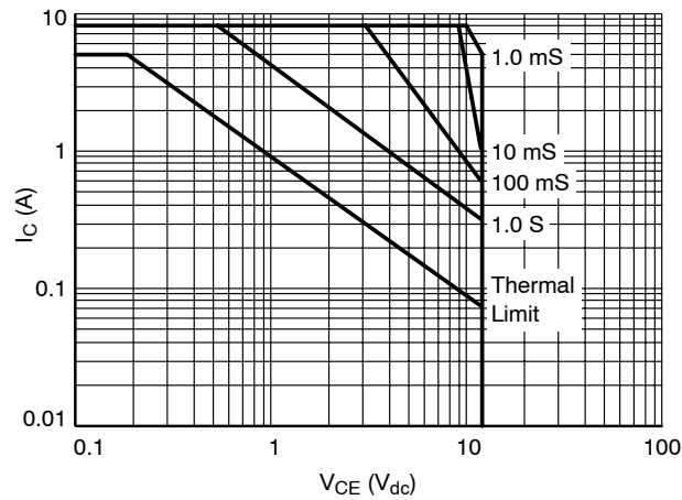
Figure 9. PNP Safe Operating Area
