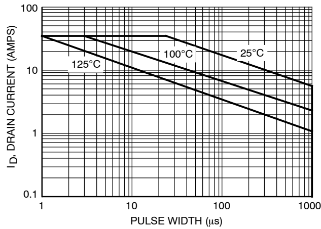
Figure 13. Avalanche Characteristics
