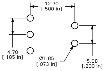
P.C. MOUNTING
