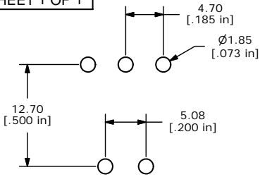
P.C. MOUNTING
