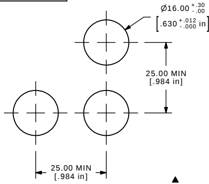
PANEL MOUNTING
