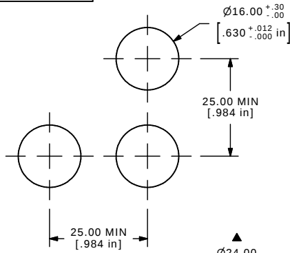
PANEL MOUNTING
