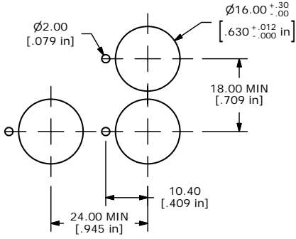
PANEL MOUNTING
