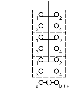
3PDT CONTACT CONFIGURATION
