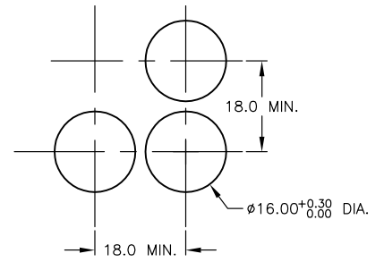
PANEL MOUNTING
