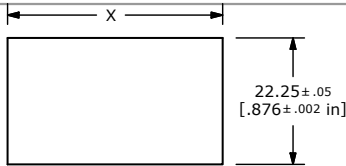
RECOMMENDED PANEL MOUNTING
