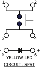
CIRCUIT: SPST
