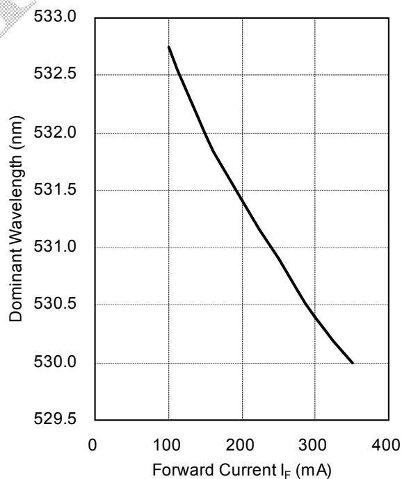
Fig 5. Wavelength Shift
