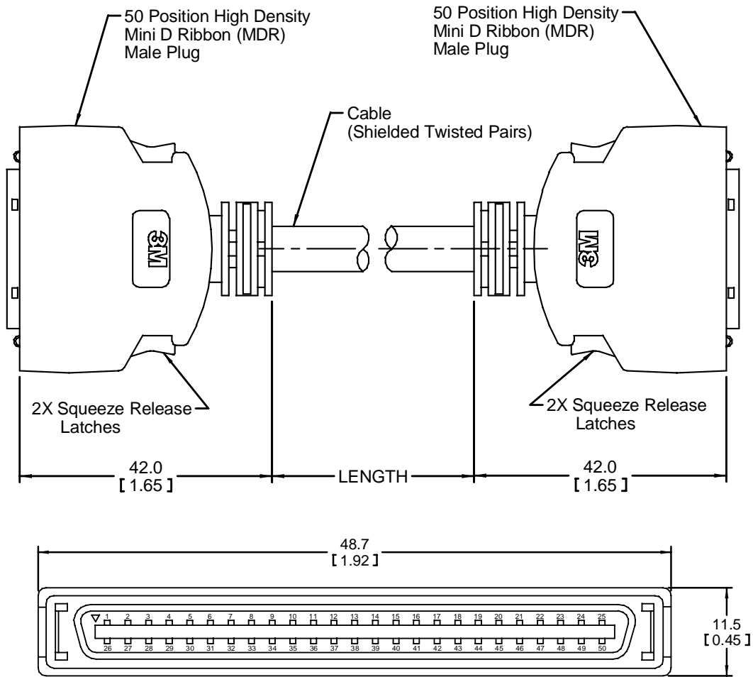
MDR 50 Position Plug Both Ends
