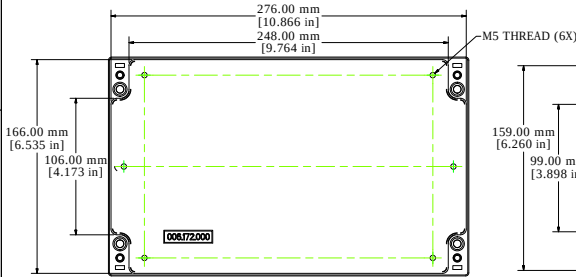
BOX - INSIDE VIEW
