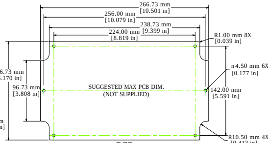
PCB
