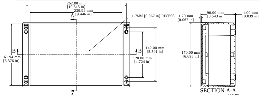
ASSEMBLY - TOP VIEW
