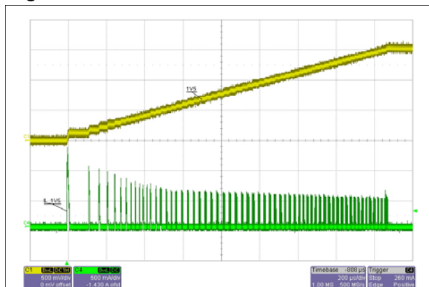
Figure 5. 1V5 soft-start without load
