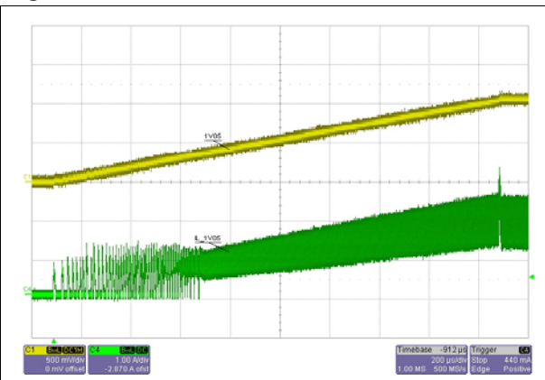
Figure 8. 1V05 soft-start without load
