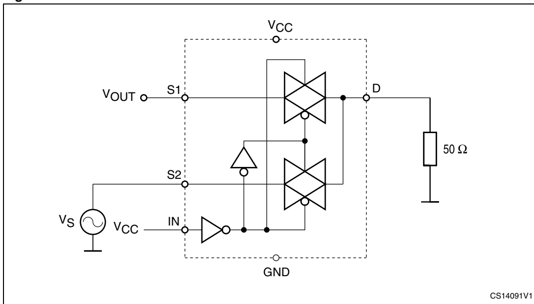
Figure 6. Channel-to-channel crosstalk
