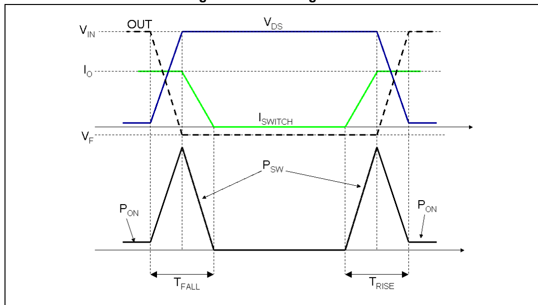
Figure 16. Switching losses
