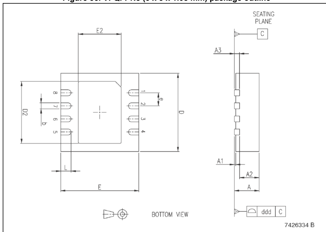
Figure 35. VFQFPN8 (3 x 3 x 1.08 mm) package outline
