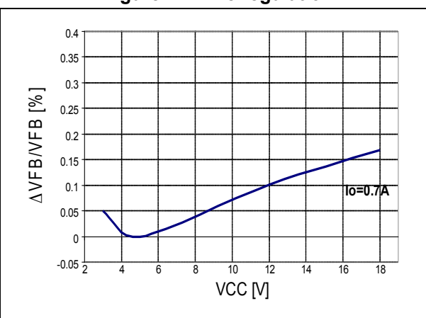
Figure 27. Line regulation
