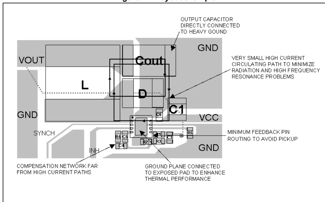
Figure 17. Layout example
