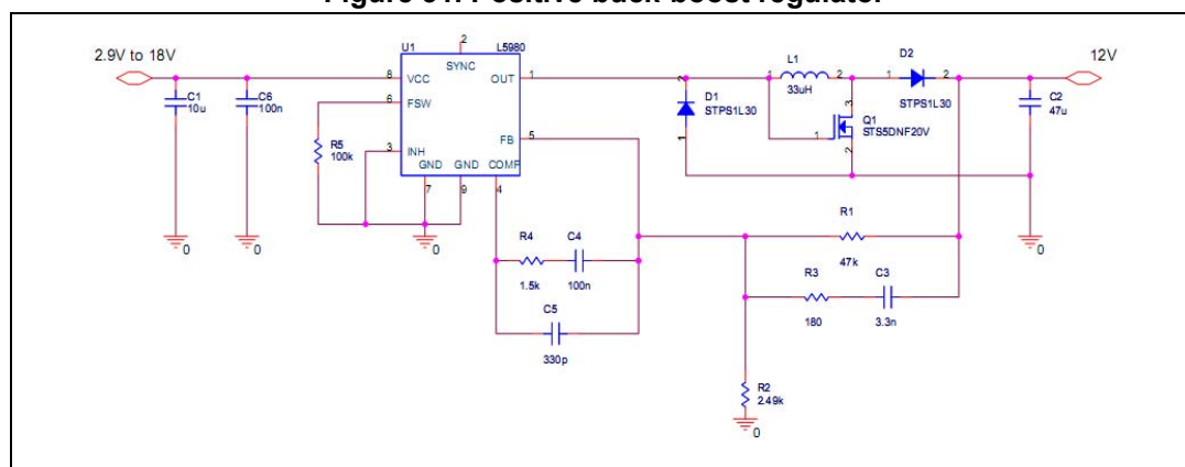
Figure 31. Positive buck-boost regulator
