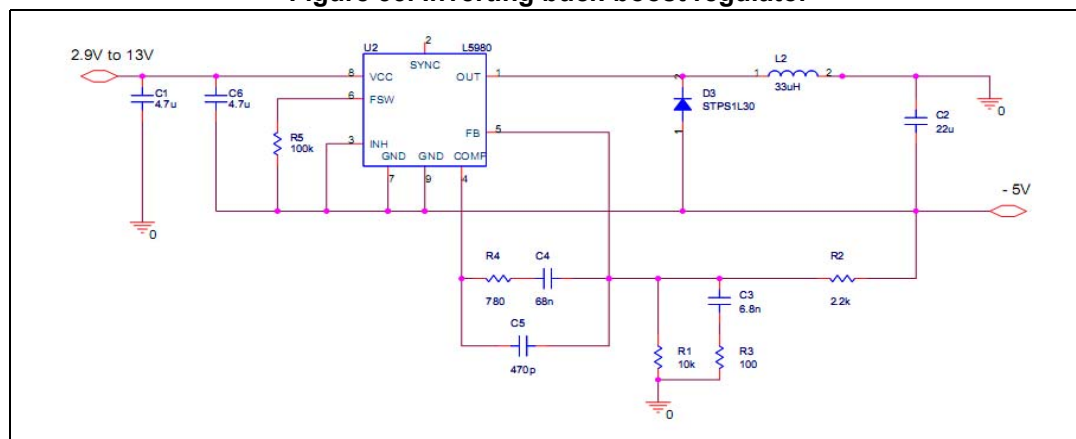
Figure 33. Inverting buck-boost regulator
