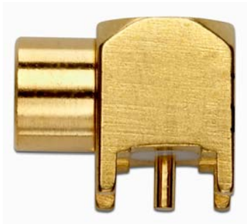
Model 73008 MCX JACK R/A PCB RECEPTACLE
