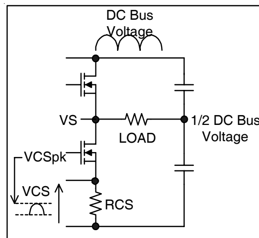
Figure 11, Calculating RCS
