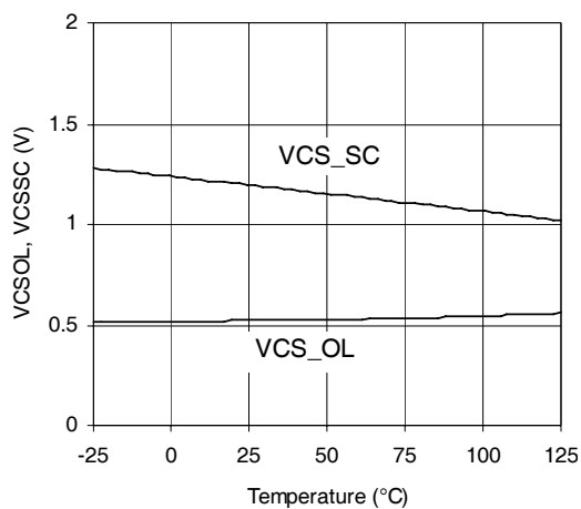
VCS_OL, VCS_SC vs TEMP (IR2161)
