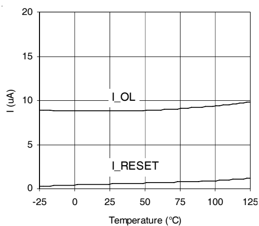
I_RESET, I_OL vs TEMP (IR2161)
