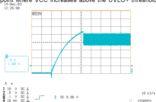
Figure 7, Startup sequence of CSD.
