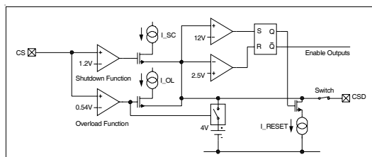
Figure 8, Shut Down Circuit.
