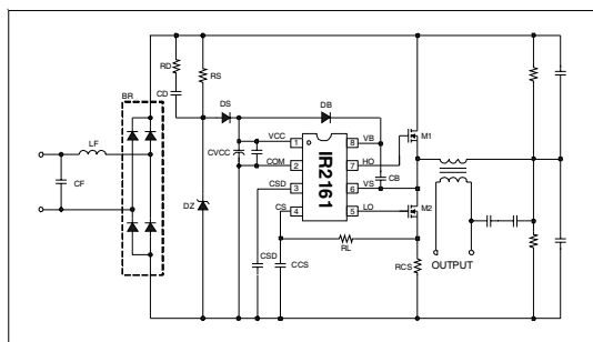
Figure 1, Halogen Converter.
