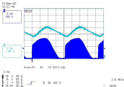
Figure 6, VS voltage and CSD voltage.
