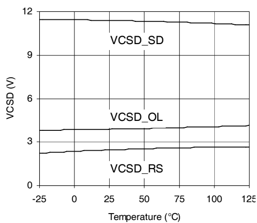
Graph : VCSDSD,OL,RS vs TEMP (IR2161)
