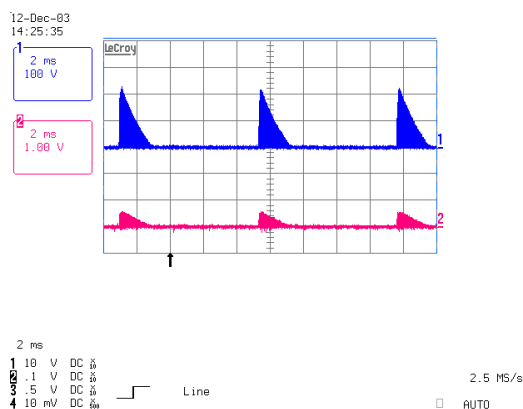
Figure 15, Half Bridge voltage and current during dimming
