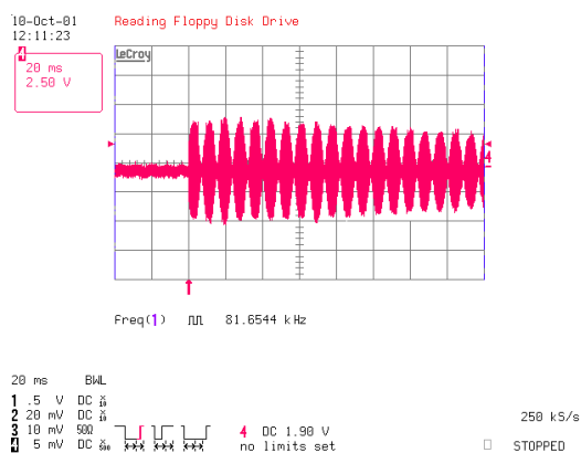
Figure 4, Cold Lamp Inrush Current with Soft Start.
