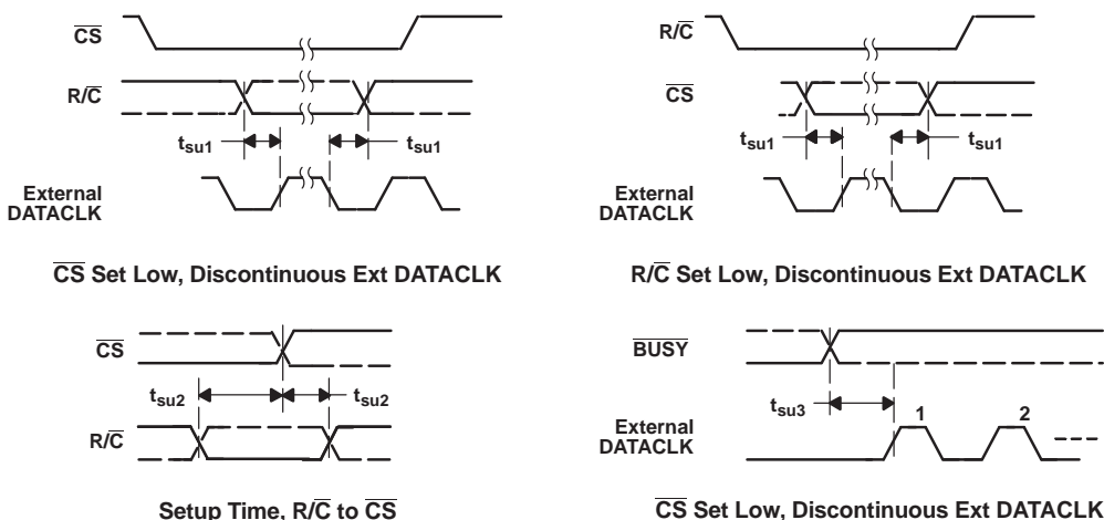
Figure 1. Critical Timing
