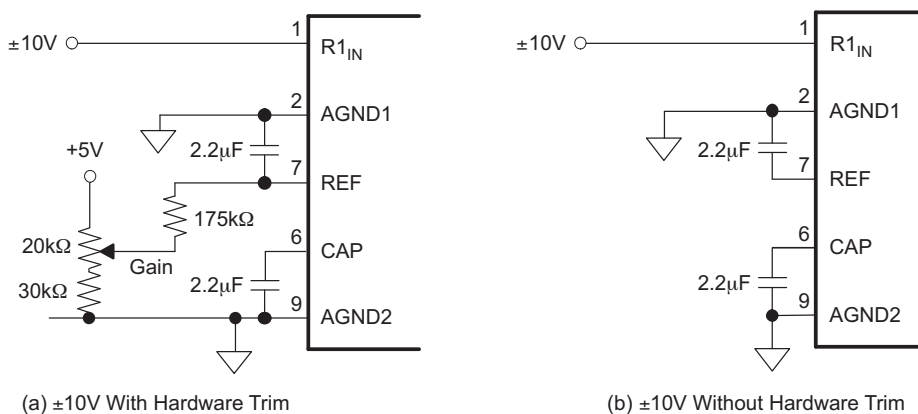
Figure 32. Gain Adjust Trim
