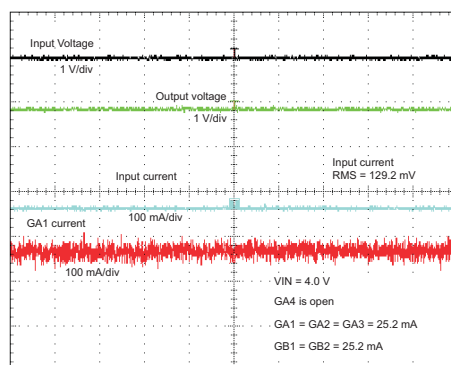
Figure 12. Open Lamp Detection (1× Mode)
