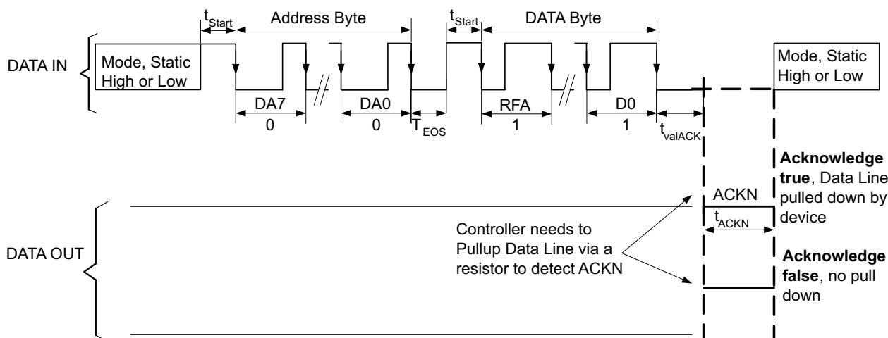
Figure 15. EasyScale Protocol With Acknowledge (RFA=1)
