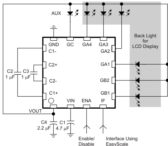
Figure 1. Typical Application
