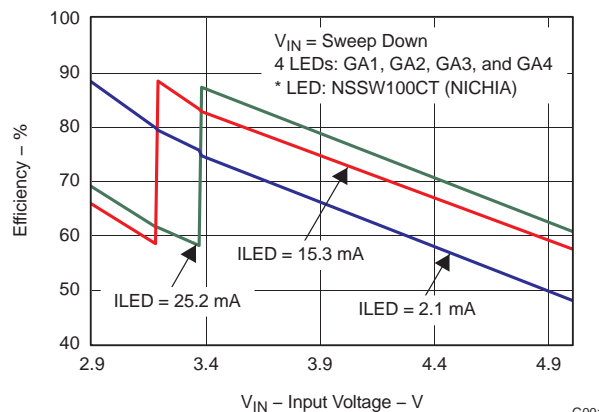
Figure 2. Characteristic Curve
