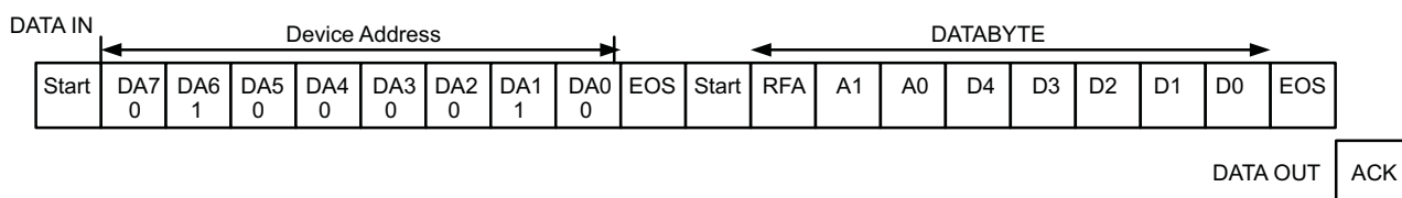
Figure 13. EasyScale Protocol Overview
