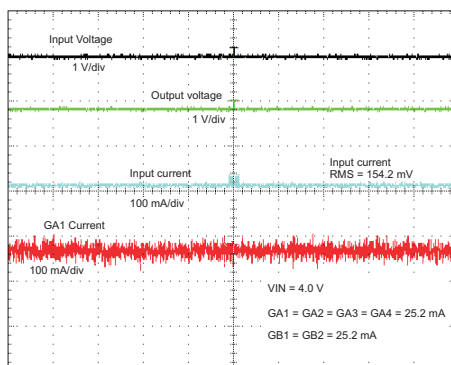
Figure 11. Normal Operation (1× Mode)
