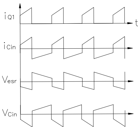
Figure 4. Typical waveforms at converter input
