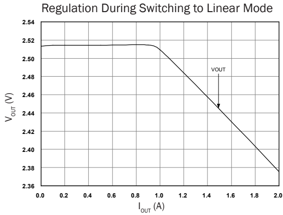
Figure 13. Loading Regulation
