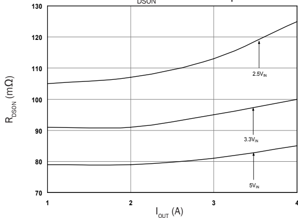
Figure 11. High-Side P-MOSFET
