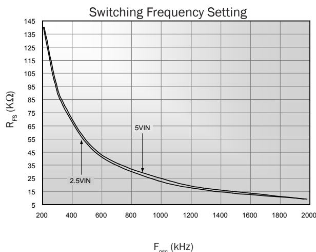
Figure 15. Switching Frequency vs. R FS
