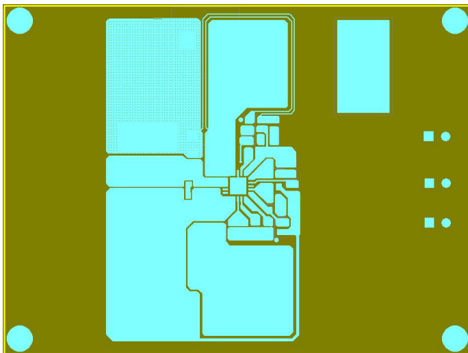
(IN1 layer)
