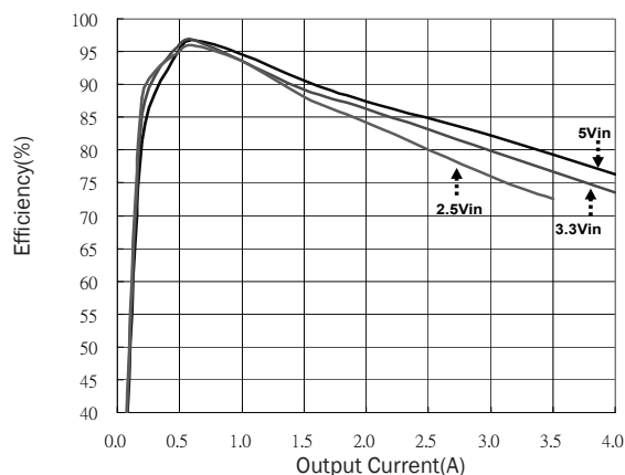
Figure 10. Efficiency(V IN )
