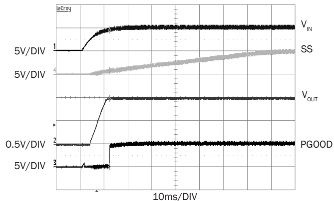
Figure 2. Start Up by V IN @4A
