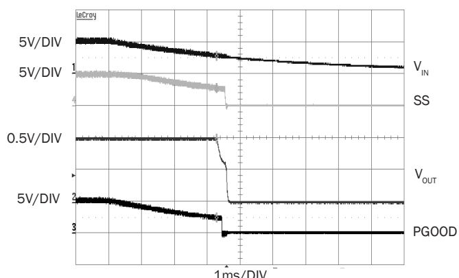
Figure 4. Shutdown by V IN @4A
