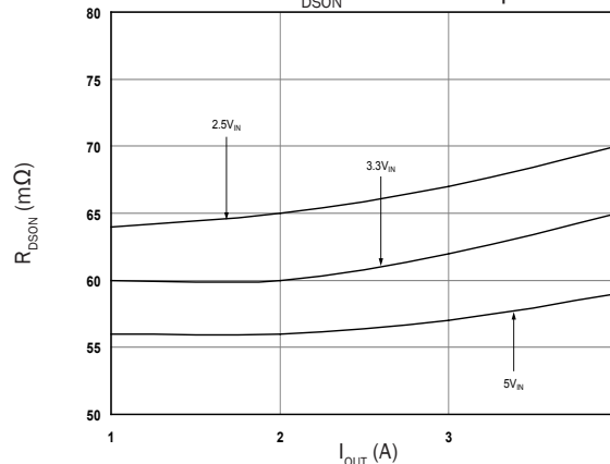
Figure 12. Low-Side N-MOSFET
