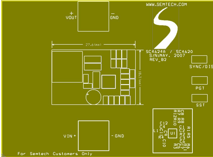
(TOP layer)
