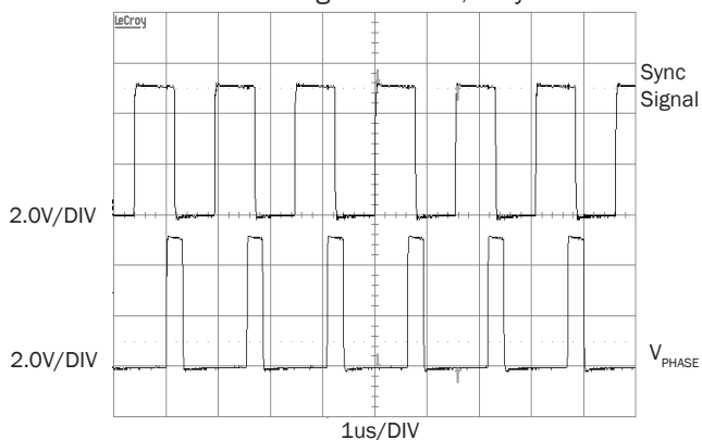
Figure 9. Synchronization
