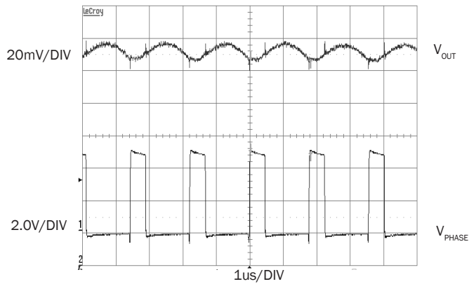
Figure 6. Ripple and Stability@4A
