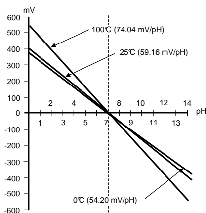
Figure 51. pH Electrode Transfer Function
