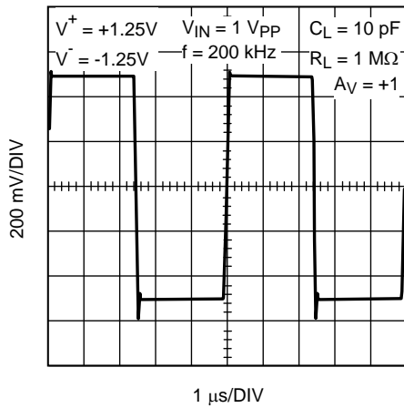
Figure 27. Large Signal Step Response
