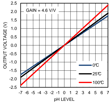
Figure 53. Output Voltage vs. pH Level
