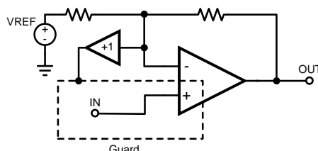
Figure 47. Guarding the Noninverting Configuration
