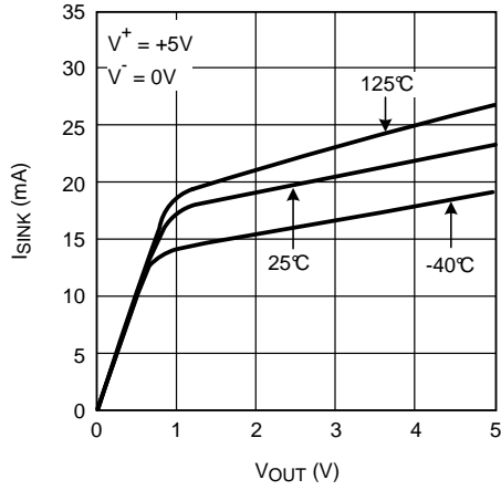
Figure 37. Sinking Current vs. Output Voltage
