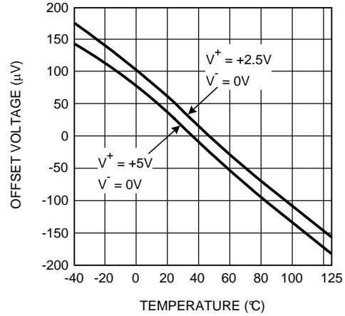
Figure 14. Offset Voltage vs. Temperature
