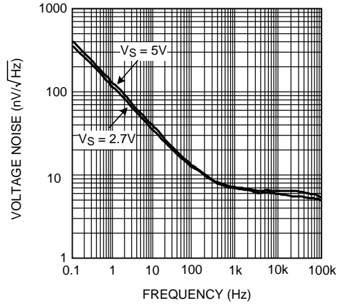
Figure 22. Input-Referred Voltage Noise vs. Frequency
