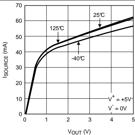
Figure 35. Sourcing Current vs. Output Voltage
