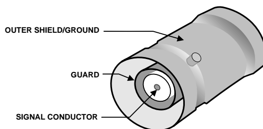
Figure 49. The Structure of a Triax
