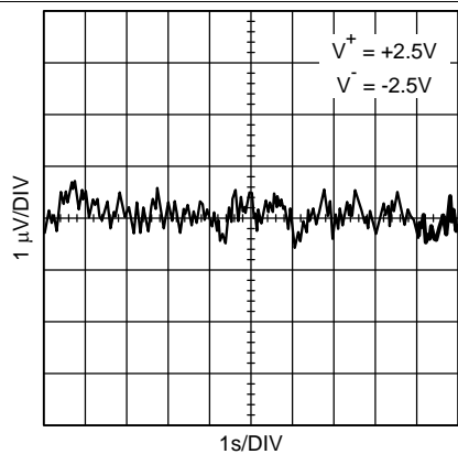
Figure 23. Time Domain Voltage Noise
