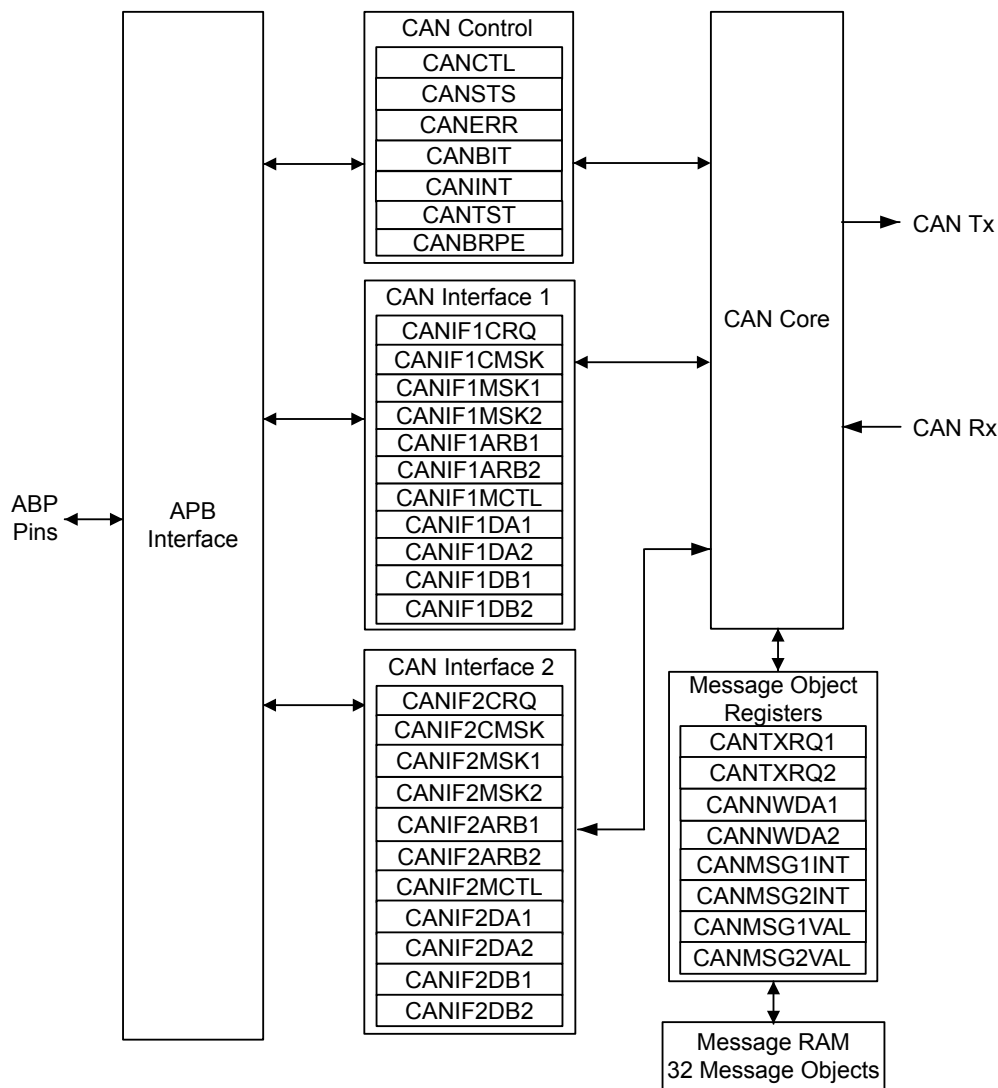
Figure 16-1. CAN Controller Block Diagram
