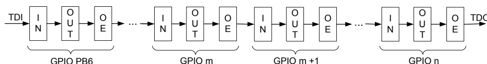
Figure 4-5. Boundary Scan Register Format
