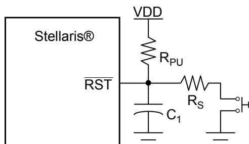
Figure 5-3. Reset Circuit Controlled by Switch
