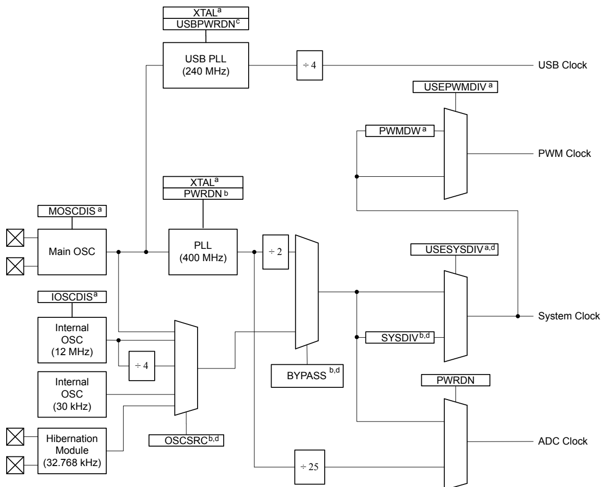
Figure 5-4. Main Clock Tree
