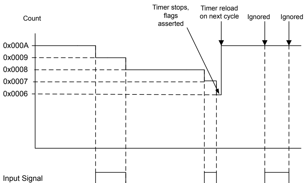
Figure 10-2. 16-Bit Input Edge Count Mode Example
