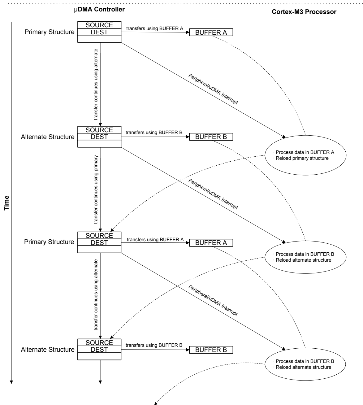
Figure 8-2. Example of Ping-Pong DMA Transaction
