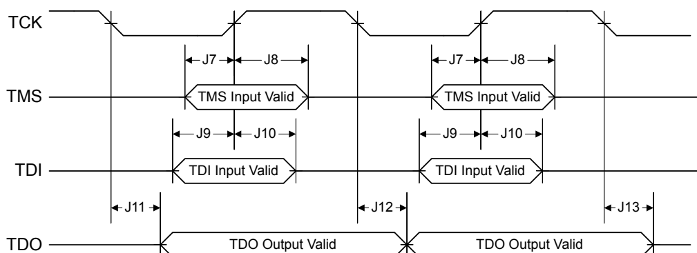
Figure 22-3. JTAG Test Access Port (TAP) Timing
