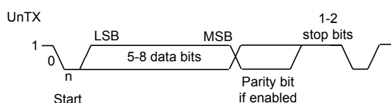
Figure 13-2. UART Character Frame
