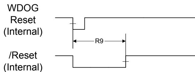
Figure 22-8. Watchdog Reset Timing
