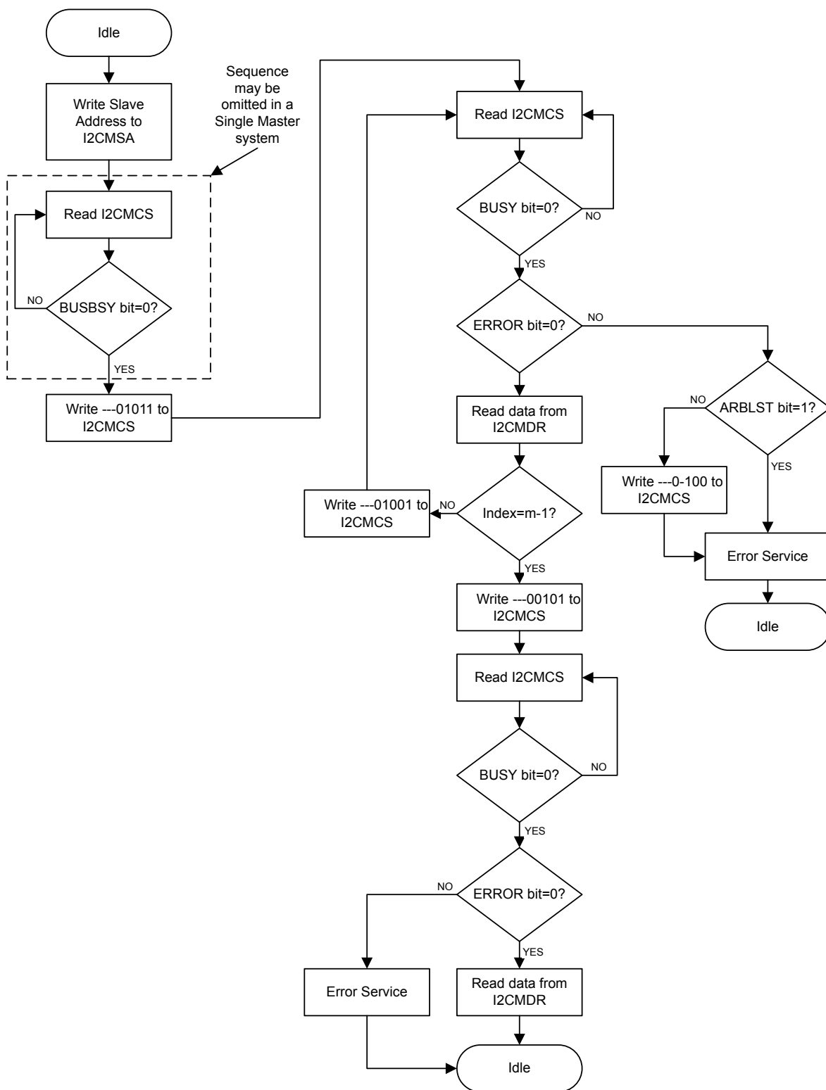
Figure 15-10. Master Burst RECEIVE
