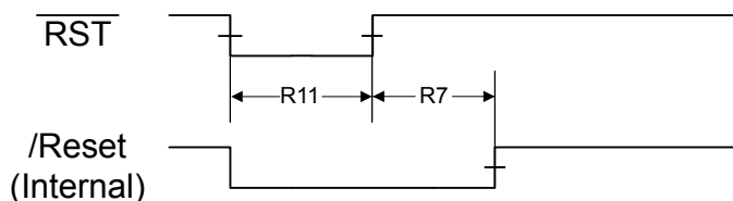
Figure 22-4. External Reset Timing ( \overline{RST} )
