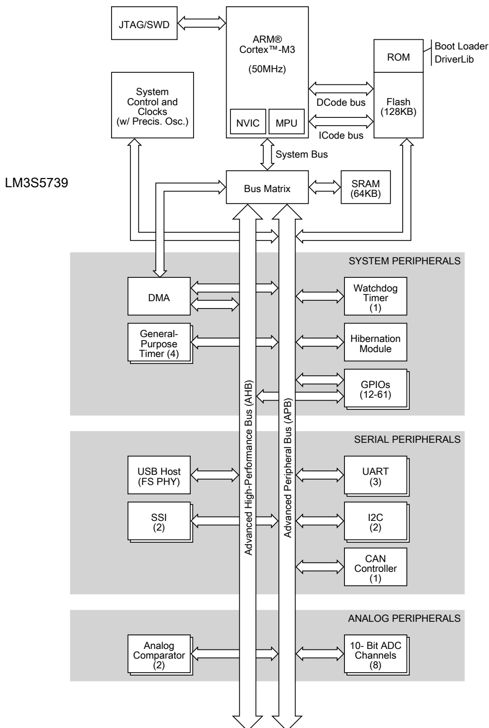
Figure 1-1. Stellaris LM3S5739 Microcontroller High-Level Block Diagram
