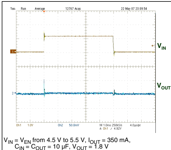
Figure 22. Line transient
