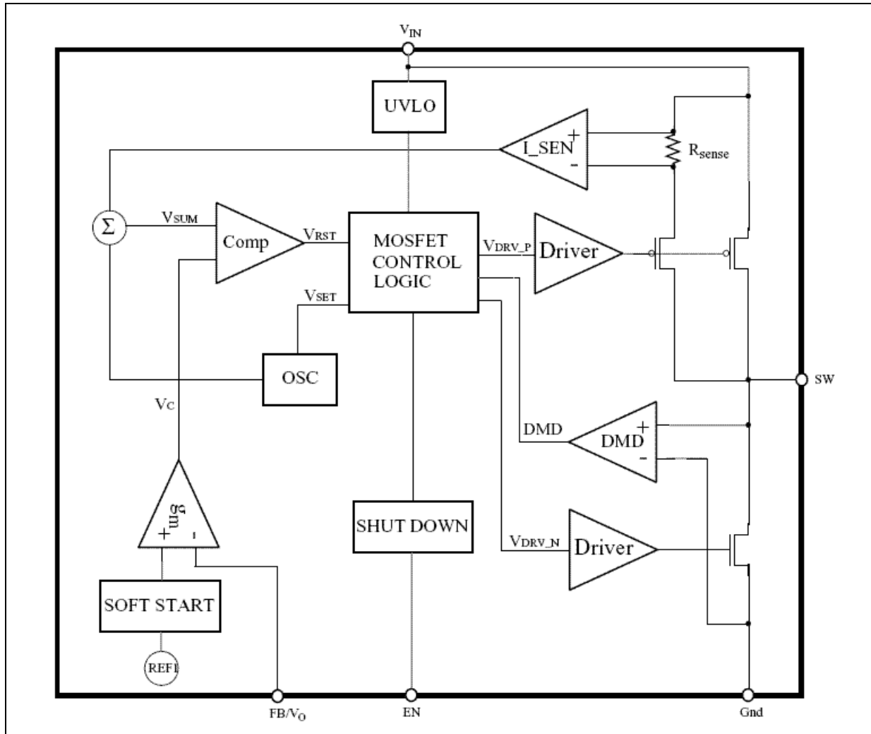
Figure 1. Schematic diagram
