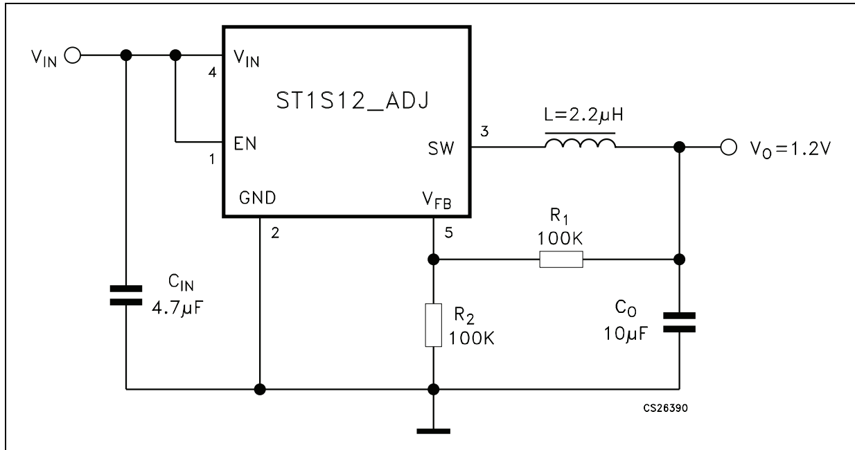
Figure 3. Application circuit
