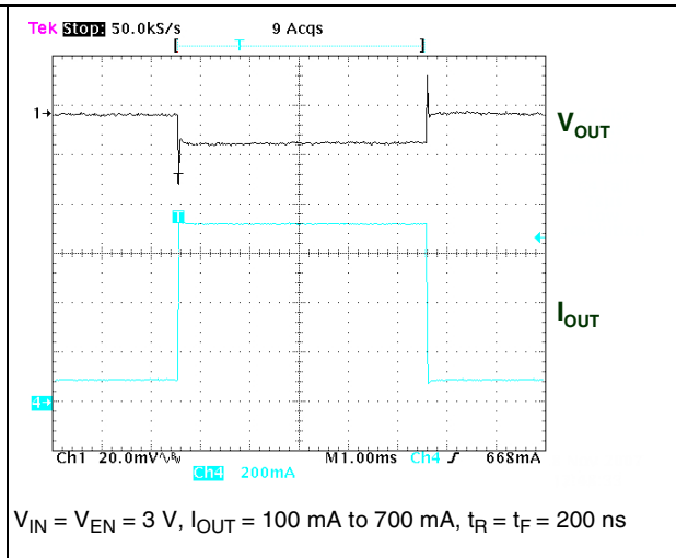
Figure 23. Load transient
