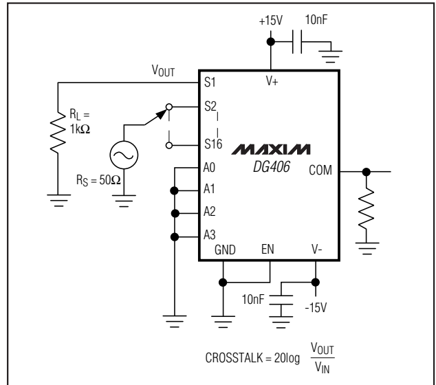
Figure 7. Crosstalk
