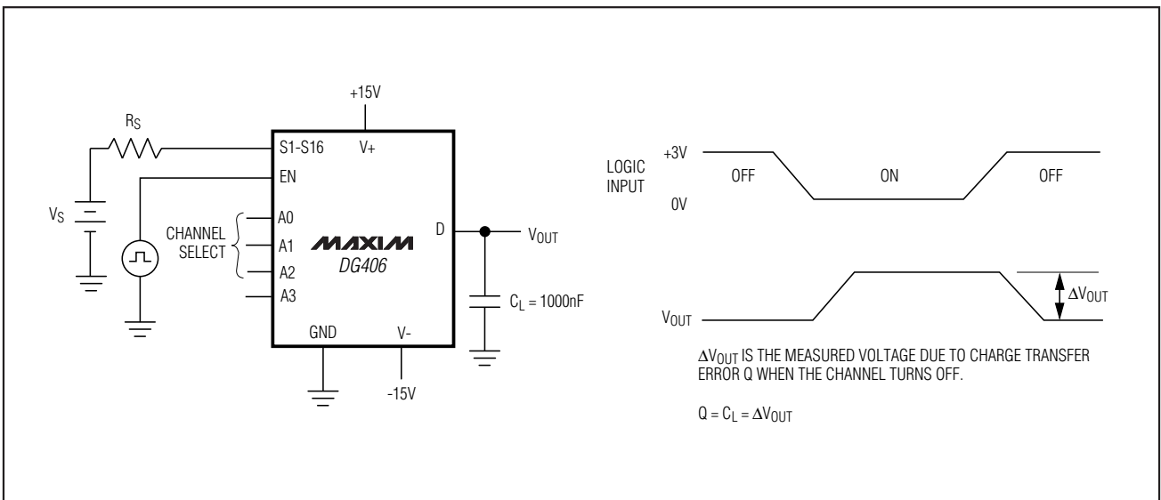
Figure 5. Charge Injection
