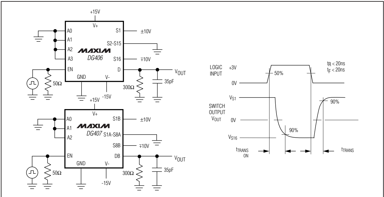
Figure 2. Transition Time
