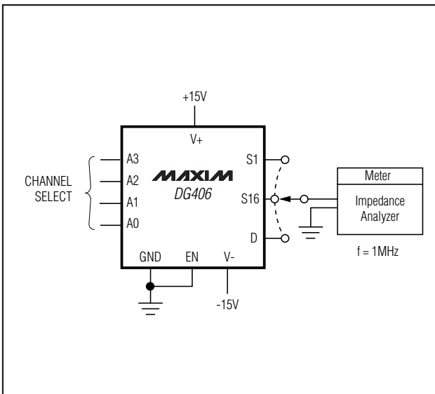
Figure 8. Source/Drain Capacitance
