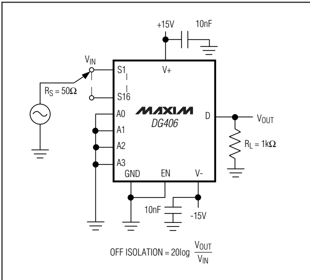
Figure 6. Off-Isolation
