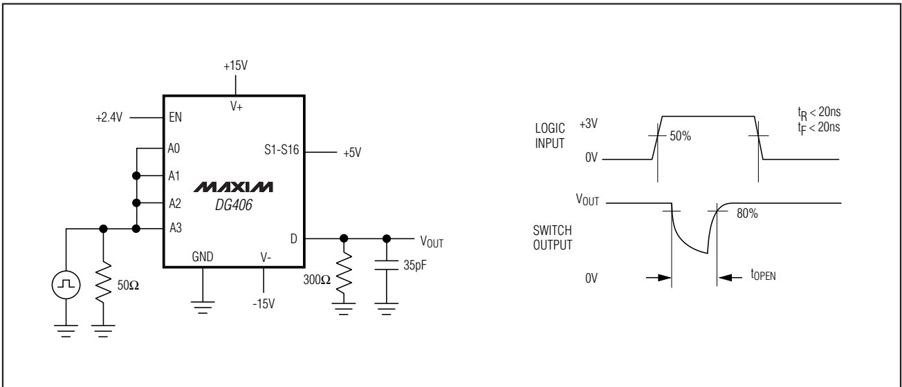
Figure 4. Break-Before-Make Interval
