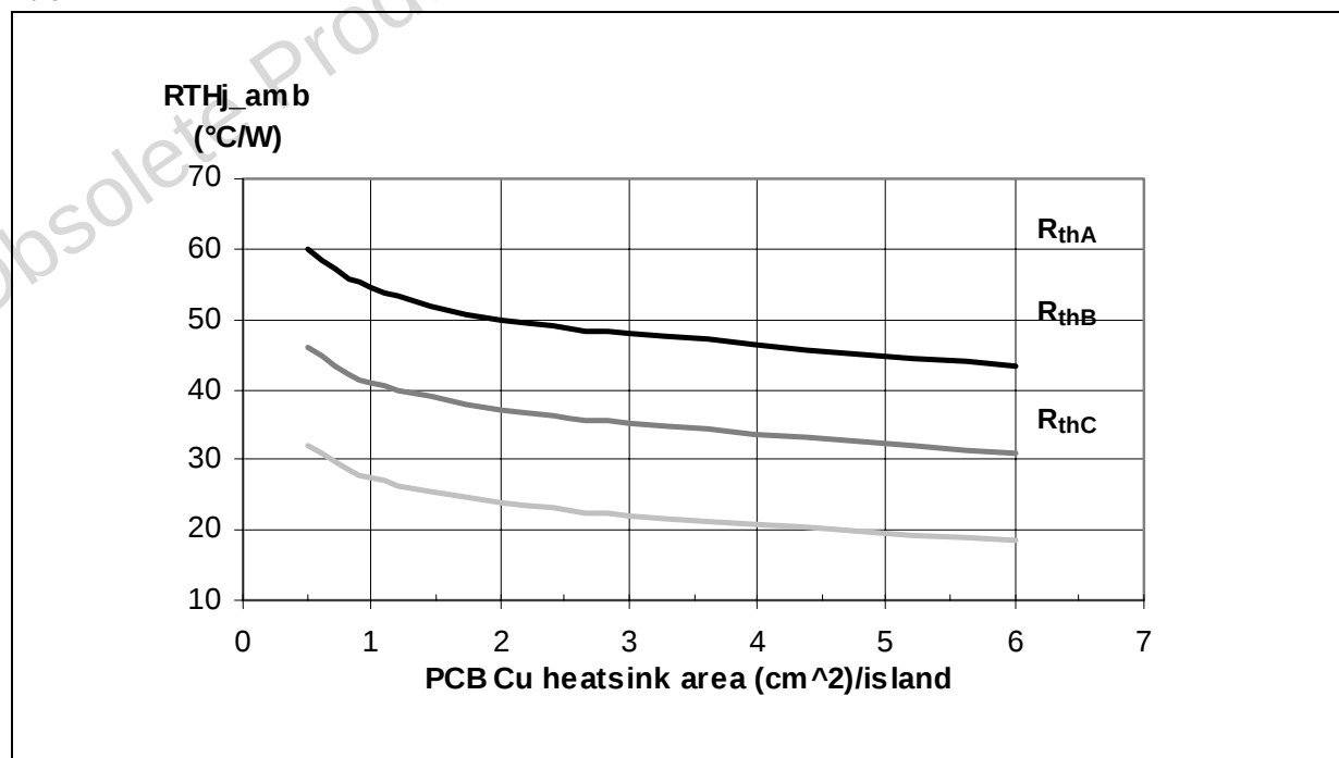
Figure 29. R_{thj-amb} Vs. PCB Copper Area In Open Box Free Air Condition
