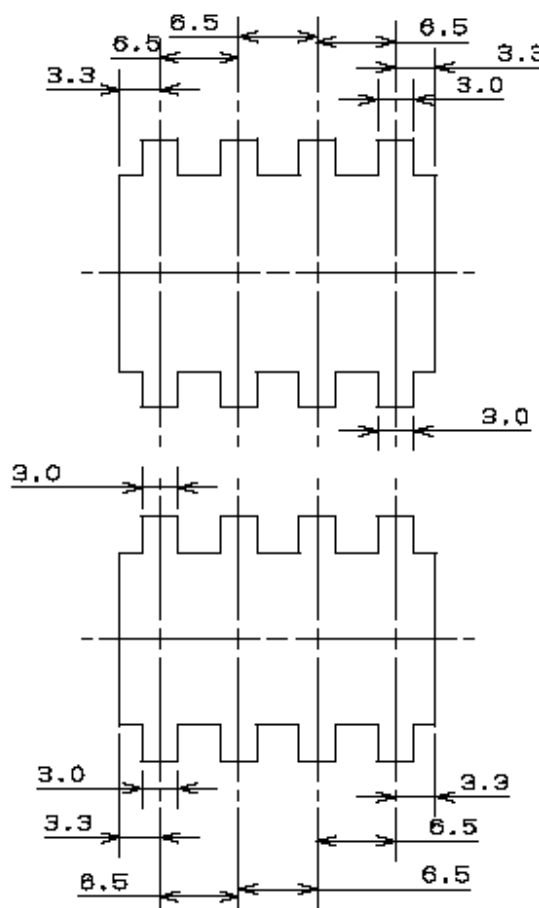
Multiple Mounting
