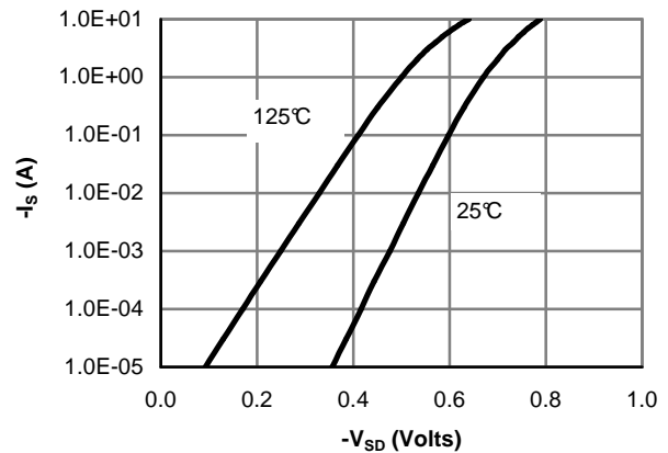
Figure 6: Body-Diode Characteristics
